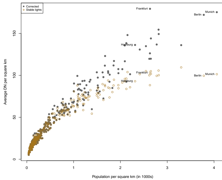
Figure H-1 – Light intensity versus population density in German regions
