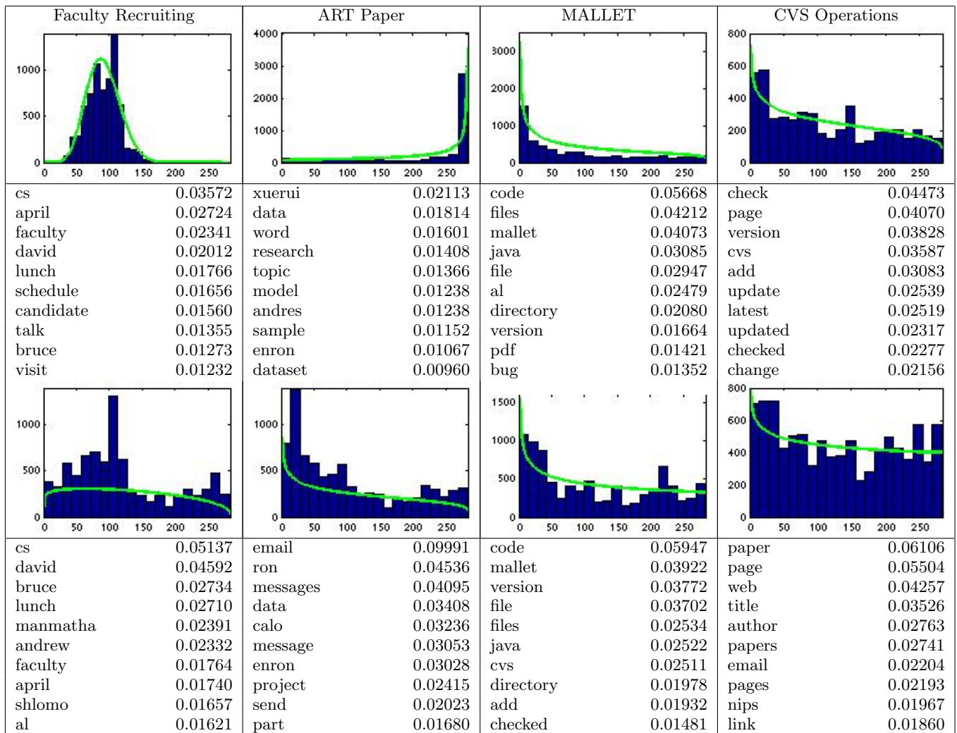
Figure 3: Four topics discovered by TOT (above) and LDA (bottom) for the Email dataset, showing improved results with TOT. For example, the Faculty Recruiting topic is correctly identified in the spring in the TOT model, but LDA confuses it with other interactions among faculty.
