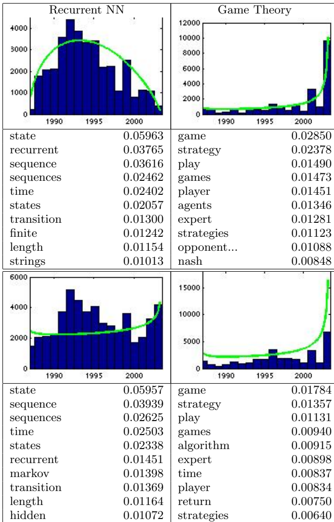
Figure 4: Two topics discovered by TOT (above) and LDA (bottom) for the NIPS dataset. For example, on the left, two major approaches to dynamic system modeling are confounded by LDA, but TOT more clearly identifies waning interest in Recurrent Neural Networks, with a separate topic (not shown) for rising interest in Markov models.
