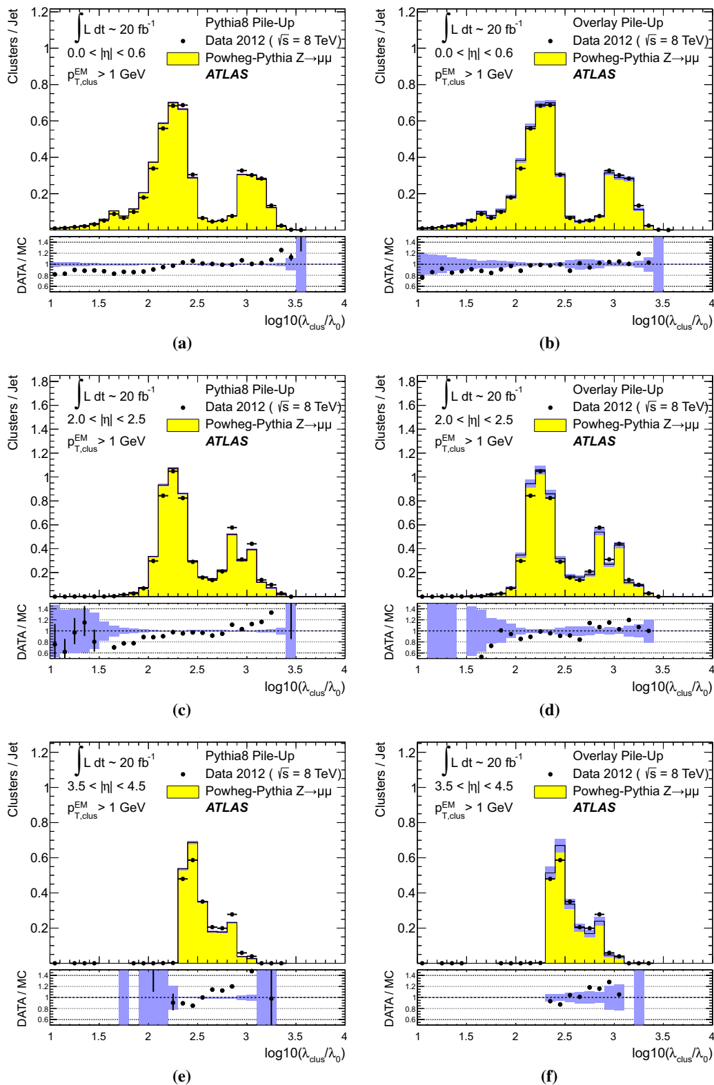
Fig. 35 The distribution of the depth location, measured in terms of \log_{10}(\lambda_{\text{clus}}/\lambda_0) with \lambda_0 = 1 mm, of topo-clusters with p_{\text{T,clus}}^{\text{EM}} > 1 GeV in jets reconstructed with the anti- k_t algorithm with R = 0.4 and with 30 \text{ GeV} < p_{\text{T,jet}}^{\text{LCW+JES}} < 40 \text{ GeV} in Z \rightarrow \mu\mu events in 2012 data and MC simulations with (a, c, e) fully simulated pile-up and with (b, d, f) overlaid pile-up from data. Distributions are shown for jets in the (a, b)
