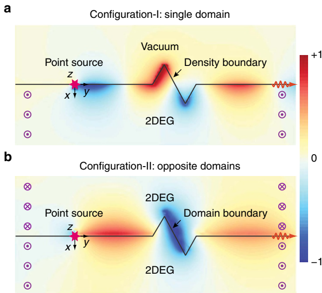
Figure 3 | Snapshots of one-way propagating topological edge states immune to backscattering at a sharp zigzag defect. Here the cyclotron frequency \omega_c = 4\omega_s , which corresponds to B_0 = 0.9 T. The driving frequency for the point source is \frac{1}{2}\omega_c , which corresponds to f = 12.7 GHz. (Refer to Methods: Theoretical model). (a) Configuration-I: a 2DEG is in contact with vacuum under a single-domain magnetic field. (b) Configuration-II: a 2DEG is uniformly filled in the whole space under an opposite-domain magnetic field. Note that the profile is plotted for the electric scalar potential, which is non-zero in the vacuum region. The difference between a and b on the wavelengths is consistent with the slightly different dispersion slope of the topological edge states between Configuration-I and II. (See online Supplementary Movies 1 and 2 for real-time evolution).
