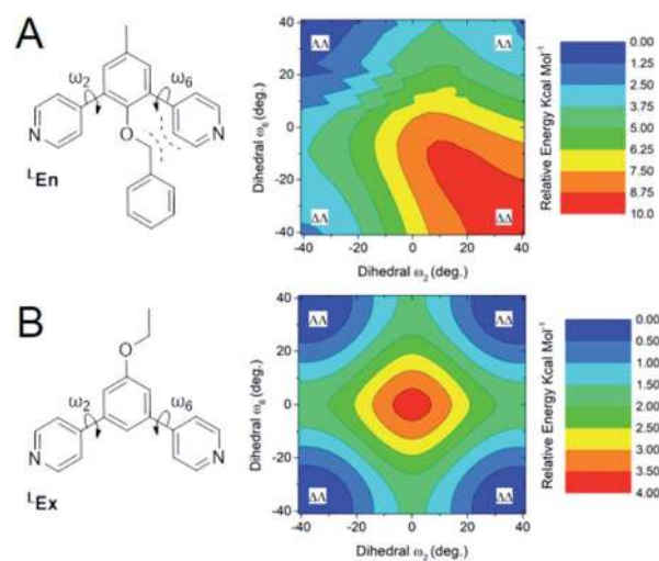
Fig. 7 Computed free energy surfaces of dihedral rotations of model systems for \text{L}^n\text{En} (A) and \text{L}^n\text{Ex} (B). Left, simple drawing of the model system showing the dihedral rotation (arrows), and expected source steric hindrance (dashed lines). Right, potential energy surfaces produced from a relaxed scan of the dihedral angles ( \omega_2 , \omega_6 ) between \pm 40^\circ from coplanarity in 28 steps of 3^\circ for each dihedral angle. These DFT calculations were conducted at a B3LYP/def2-TZV level of theory, with the color contour corresponding to the relative free energy of each dihedral pair in kcal mol -1 .
