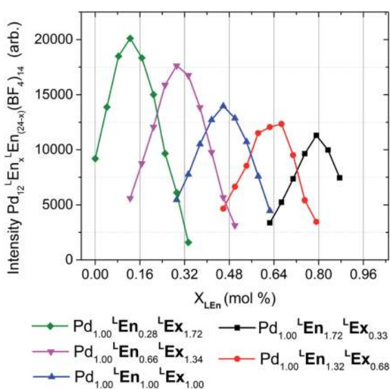
Fig. 6 Distributions of heteroleptic assemblies observed by ESI-HRMS. Assembly product mixtures were formed in deuterated acetonitrile from 10.0 mM total concentration of \text{L}^n\text{En} and \text{L}^n\text{Ex} with 5.0 mM of \text{Pd}(\text{BF}_4)_2 and were directly analyzed without dilution by ESI-HRMS. The observed mass spectra of \text{Pd}_{12}\text{L}^n\text{En}_x\text{Ex}_{(24-x)}(\text{BF}_4)_{14}^{10+} species suggests a single product topology. These results are further detailed in the ESI (Section H†).
