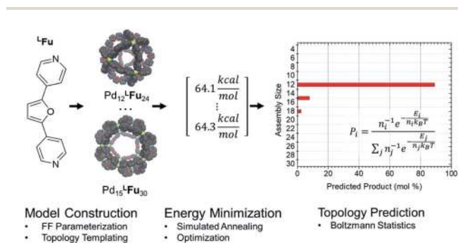
Scheme 1 Flow chart for topological prediction of homoleptic assemblies featuring the formation of homoleptic Pd x 1 Fu 2x assemblies. The linker structure is used to construct a library of possible assembly outcomes, which are subjected to a simulated annealing and structural optimization procedure using implicit solvation. The resulting minimum energies, E_i are treated as microstates, and the topological distribution is determined using Boltzmann statistics with a weighting factor ' n ' corresponding to the number of linker components in the assembly.
