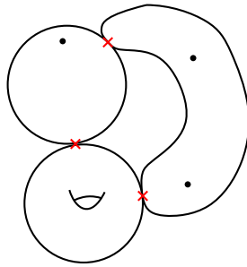
Figure 3: A nodal Riemann surface in \partial \overline{\mathcal{M}}_{2,3} . It has three smooth components which have genus/number of punctures and nodes (0,3) , (0,4) , (1,2) , hence they all have finite automorphism group.
