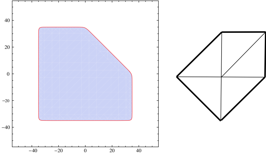
FIGURE 1. The figure on the left shows the region (2.46) in phase space for the quantum operator associated to local \mathcal{B}_2 , for E = 35 and m_1 = m_2 = 1 . The figure on the right is the polyhedron representing toric \mathcal{B}_2
