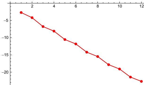
FIGURE 4. The difference \Delta(4\pi, m) , defined in (4.27), for the local \mathbb{P}^2 geometry
