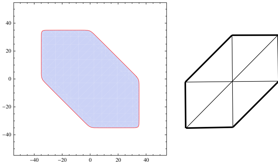
FIGURE 2. The figure on the left shows the region (2.46) in phase space for the quantum operator associated to local \mathcal{B}_3 , for E = 35 and m_1 = m_2 = m_3 = 1 . The figure on the right is the polyhedron representing toric \mathcal{B}_3
