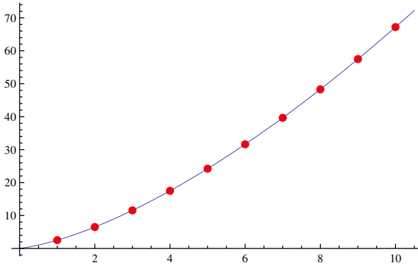
FIGURE 6. The smooth line gives the free energy F(N, 2\pi) of local \mathbb{F}_1 as a function of N , computed from (3.47), while the points give the values of of the free energy as computed from the spectral traces
