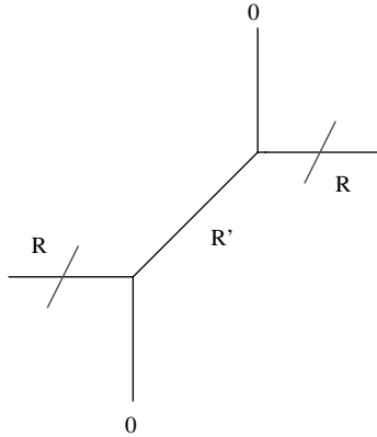
Figure 4: Toric graph of the blowup \mathcal{X}_0 \rightarrow X_0 . The dashes indicate that the horizontal edges (labelled R ) are identified. The diagonal edge (labelled R' ) is the new \mathbb{P}^1 at the origin of X_0 .
