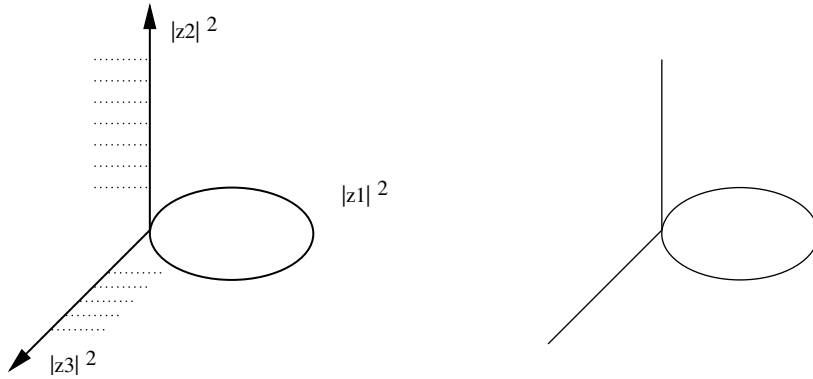
Figure 3: Toric construction of the fibration X_0 .
