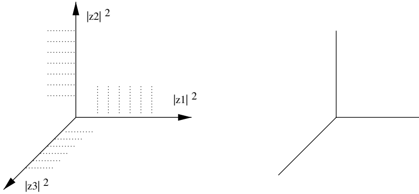
Figure 2: \mathbb{C}^3 as a toric fibration.
