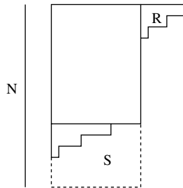
Figure 1: Coupled representations with S = R_+ and R = R_- .
