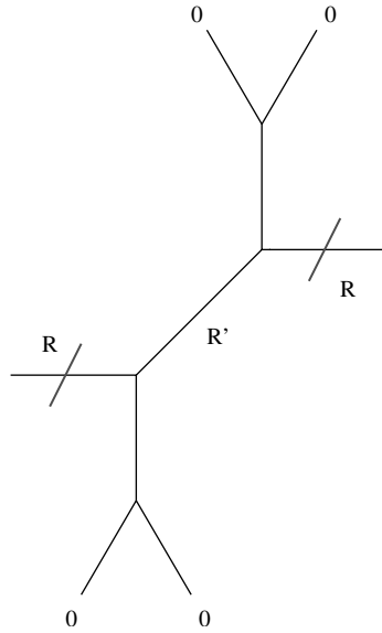
Figure 5: The formal toric geometry arising in the topological quantum field theory.
