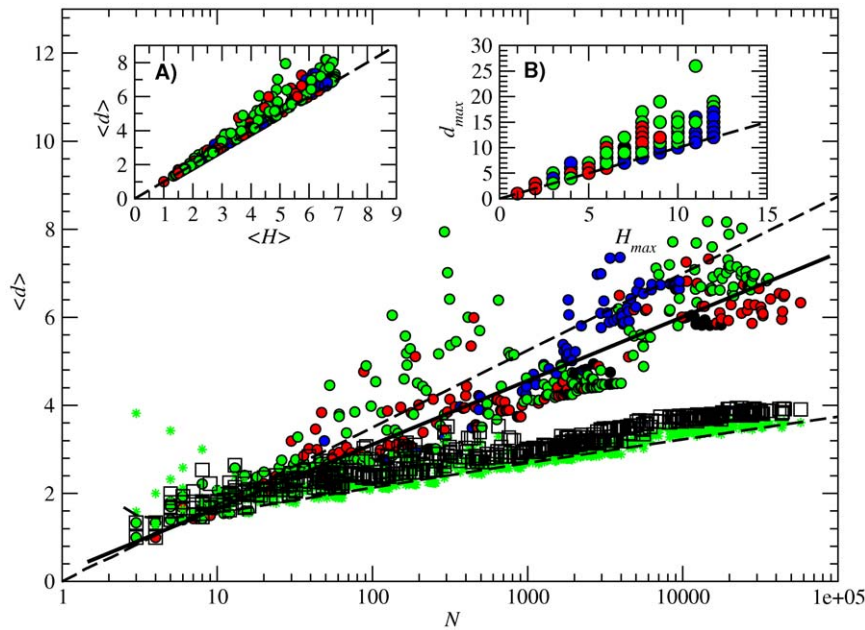
Figure 7. Average shortest path \langle d \rangle . Dependence of the average shortest path on the subnetwork size N for all folded neutral networks (colored circles), equivalent random networks (black squares) and theoretical predictions with a classical random model ( \langle d \rangle \sim \ln N / \ln \langle k \rangle , green stars). Circle colors correspond to the number of base pairs of each subnetwork (see caption of Fig. 3). The numerical fitting is plotted as a solid black line, while the analytical approximations correspond to the long-dashed black lines (for values of \alpha and A_S numerically obtained from the folding of all 12-nt sequences). Inset (A): relation between the average shortest path \langle d \rangle and the average Hamming distance \langle H \rangle of the subnetworks. Inset (B): relation between the longest distance between any pair of nodes of the network d_{max} and the maximum number of different bases between sequences H_{max} (maximum Hamming distance). In the insets, the dashed lines are \langle d \rangle = \langle H \rangle and d_{max} = H_{max} , which correspond to the lower bounds of \langle d \rangle and d_{max} , respectively. doi:10.1371/journal.pone.0026324.g007
