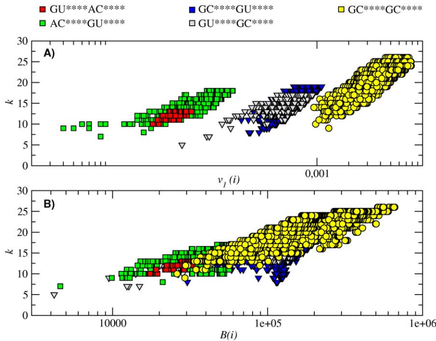
Figure 9. Sequence centrality. Evaluation of the sequence centrality for the largest subnetwork N=57481 , whose secondary structure is ((...)).... In (A), degree k_i versus eigenvector centrality v_1(i) . In (B), degree k_i versus betweenness centrality B(i) . Colors and shapes denote the type of base pairs the sequences have (see Figure's legend). Note the community division created by the eigenvector centrality, which is related to the type of nucleotides participating in the base pair: GC+UA and AU+CG for low eigenvector centrality, GU+CG and GC+UG and for intermediate v_1(i) and GC+CG for high v_1(i) . doi:10.1371/journal.pone.0026324.g009
