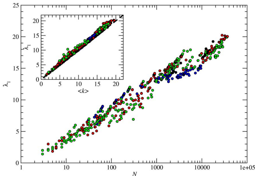
Figure 8. Eigenvector centrality. Largest eigenvalue \lambda_1 of the adjacency matrix \mathbf{A} as a function of the network size N . The inset shows the linear relationship between \lambda_1 and the network average degree \langle k \rangle . Solid line in the inset is \lambda_1 = \langle k \rangle . doi:10.1371/journal.pone.0026324.g008
