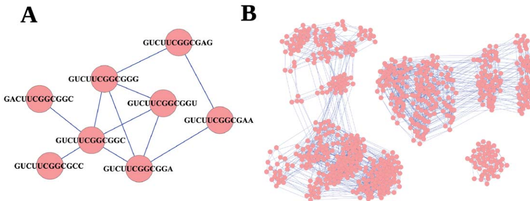
Figure 1. Construction of neutral networks. In (A), we show an example of how neutral networks are constructed: sequences that fold into the same secondary structure are connected if they are at a Hamming distance of one. In (B), we show all sequences of length 12 that fold into the secondary structure ((.....)) , which is ranked in the 46th position. Although all sequences fold into the same secondary structure, the neutral network splits into 3 isolated subnetworks of sizes N=404, 341, \text{ and } 55 . doi:10.1371/journal.pone.0026324.g001
