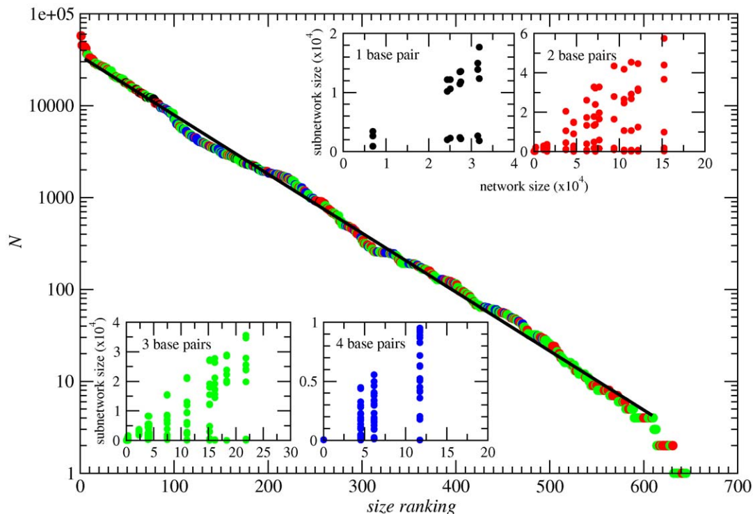
Figure 2. Subnetworks size ranking. In linear-logarithmic scale, ranking distribution of subnetwork sizes. Colors indicate the number of base pairs L_p in the secondary structure: one pair (black), two pairs (red), three pairs (green) and four pairs (blue). The solid line corresponds to an exponential fitting. Insets show for each group of structures (with the same L_p ) the size of the subnetworks (in the y-axis) that belong to the same neutral network as a function of the corresponding neutral network size (in the x-axis). Note changes of scale in both axes.
