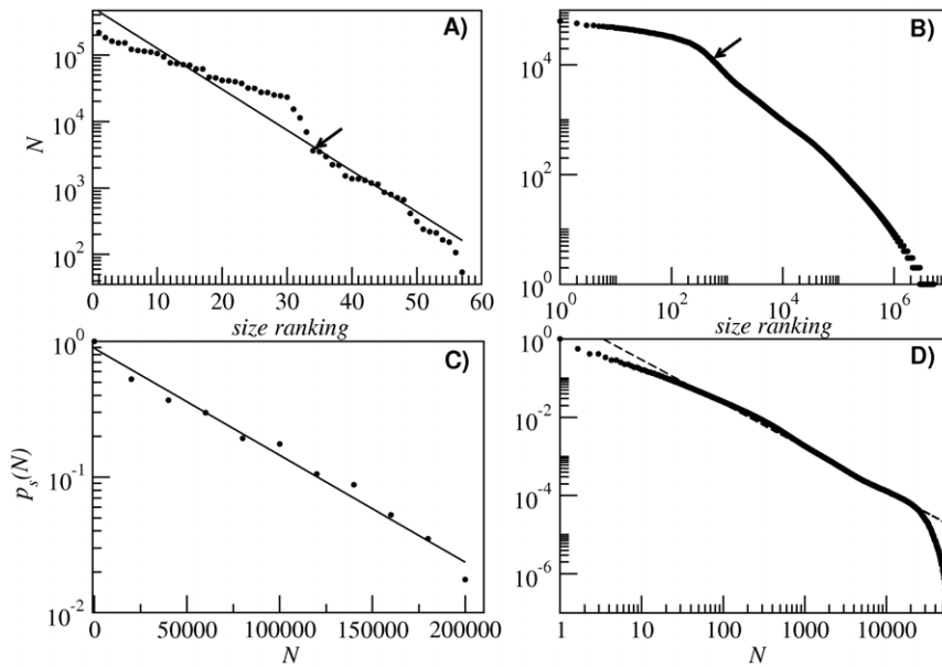
Figure 10. Comparison between l=12 and l=35 neutral networks. Rank ordering of network sizes for l=12 (A) and l=35 (B). Black arrows signal the first non-stem-loop structure. Network size abundance for l=12 (C) and l=35 (D). The solid lines correspond to exponential fits, while the dashed line corresponds to a logarithmic decay. Data for l=35 after [13]. doi:10.1371/journal.pone.0026324.g010
