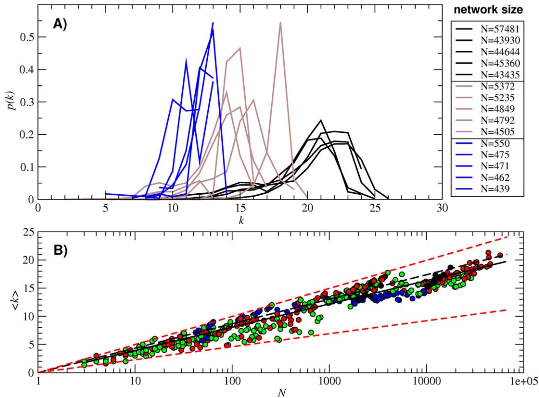
Figure 3. Degree distribution p(k) and average degree \langle k \rangle . (A) Degree distribution p(k) of fifteen subnetworks. They are the five largest (black curves), five of intermediate size (brown curves, one order of magnitude smaller) and five small subnetworks (blue curves, two orders of magnitude smaller). (B) Average degree \langle k \rangle as a function of the subnetwork size N . Colors correspond to one (black), two (red), three (green) and four (blue) base pairs in the secondary structure. The solid line corresponds to the numerical fitting \langle k \rangle \sim 1.79 \ln N (note the logarithmic-linear scale). The analytical approximation to \langle k \rangle making use of the values of \bar{u} , \bar{p} and \alpha obtained from all the 12-nt folded sequences (and implying A_S = 0.53 ) is plotted in long-dashed black line. The upper and lower bounds to coefficient A_S yield \langle k \rangle = \ln N and \langle k \rangle = (3/\ln 4) \ln N (plotted in short-dashed red lines).
