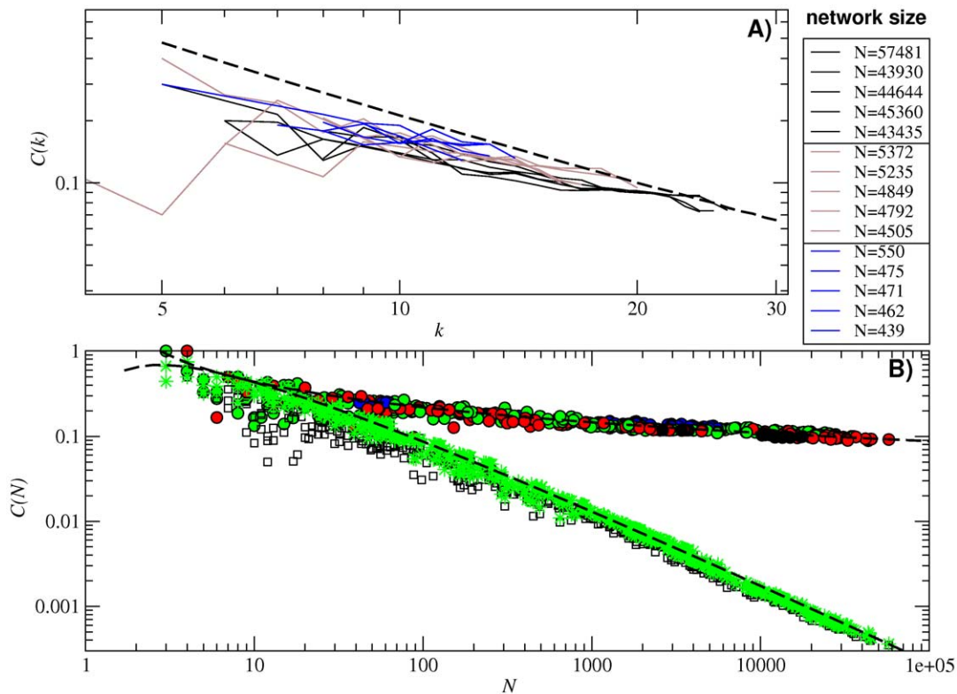
Figure 4. Clustering. (A) Clustering distribution C(k) for the fifteen networks analyzed in Fig. 3. (B) Average clustering C(N) as a function of the subnetwork size N for all folded neutral networks (colored circles), equivalent random networks (black squares) and theoretical predictions with a classical random model ( C(N) \simeq \langle k \rangle N^{-1} , green stars). Circle colors correspond to the number of base pairs of each subnetwork (see caption of Fig. 3). In both plots (A) and (B), the analytical approximations using the values of \bar{u} , \bar{p} and \alpha obtained from all the 12-nt folded sequences are plotted in long-dashed black lines.
