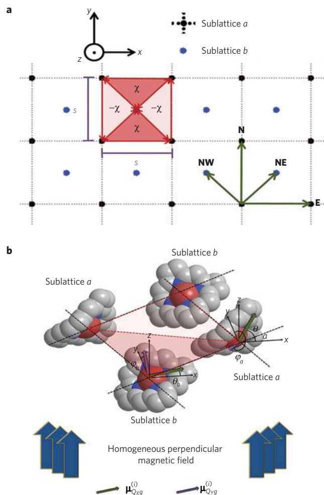
Figure 1 | Porphyrin lattice under a uniform magnetic field. a , The square lattice consists of porphyrins arranged into two sublattices a (black) and b (blue). A possible unit cell is a square of dimensions s × s . We highlight the fluxes (Berry phases) ± \chi that the exciton obtains on anticlockwise circulation about each of the minimal three-porphyrin loops. This pattern of fluxes is reminiscent of Haldane’s model, where electrons are placed in a lattice under an inhomogeneous magnetic field with no effective magnetic field per unit cell and, yet, manifest non-trivial topological properties. Dipolar coupling between a pair of porphyrins occurs along the N (north), E (east), NE (northeast) and NW (northwest) directions, as well as their opposite counterparts. b , Magnification of the upper corner of the unit cell in a . The actual set-up uses a homogeneous magnetic field. Sublattice a differs from sublattice b by the orientation angles \theta_i, \varphi_i ( i = a, b ) of the porphyrins with respect to the x and y axes. Each porphyrin consists of two transition dipoles \mu_{QXg}^{(i)} and \mu_{QYg}^{(i)} in the plane of the molecules. The anisotropic character of dipolar interactions together with the magnetic field makes the exciton hoppings along the northeast and the northwest directions different enough to obtain a non-zero flux \chi .
