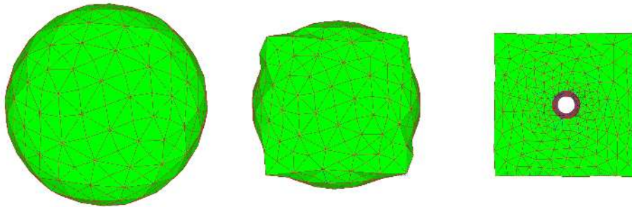
Fig. 9: Reconstruction of an artificial point cloud – a box with a cylindrical tunnel.
