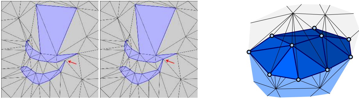
Fig. 1: Interface representation in the deformable simplicial complex (2D on the left, 3D on the right). Exterior triangles (tetrahedra) are light gray, interior – blue. Simplices belonging to the interface (edges and vertices in 2D; faces, edges and vertices in 3D) are highlighted in dark blue. On the left, the red arrow indicates where a topological change takes place. Note also the difference in scale between the largest and the smallest triangles.
