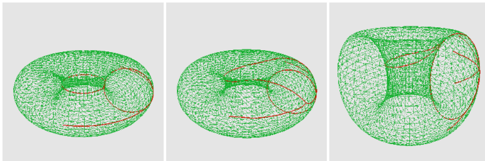
Fig. 7: 2D DSC-based cut locus construction algorithm results for tori: left and middle – cut loci of a standard torus of revolution with circular generator \mathbf{r}_1(u, v) = ((2 + \cos(v)) \cos(u), (2 + \cos(v)) \sin(u), \sin(v)) , for points (u, v) = (0, 0) and (0, 0.1\pi) ; middle and right – cut locus of a standard torus of revolution with elliptic generator \mathbf{r}_2(u, v) = ((2 + \cos(v)) \cos(u), (2 + \cos(v)) \sin(u), 2 \sin(v)) , for a point (u, v) = (0, 0.1\pi) .
