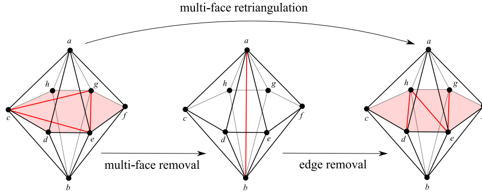
Fig. 2: Topological operations ( swaps ) used for mesh reconnection in 3D DSC. Each operation is performed only if it improves the minimum quality locally.
