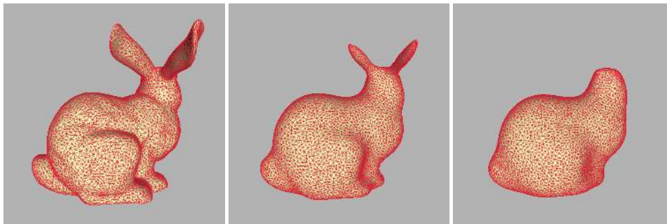
Fig. 4: Mean curvature flow quickly erases high frequency details of the surface. Note an important property of the DSC – the interface mesh only changes in the regions where it is needed, in order to accommodate the deformation. One can notice that most of the triangulation remains essentially unchanged between the frames, except for the ears, where the triangulation changes a lot (since this part of the mesh is affected the most by the mean curvature flow). The bunny model is courtesy of the Stanford 3D scanning repository.
