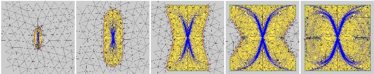
Fig. 8: A few steps of the cut locus construction algorithm for a standard torus of revolution. An equidistant front (highlighted in red) is propagating along geodesics (highlighted in blue) in the (u, v) -plane. Whenever the front collides with itself it stops (highlighted in green).
