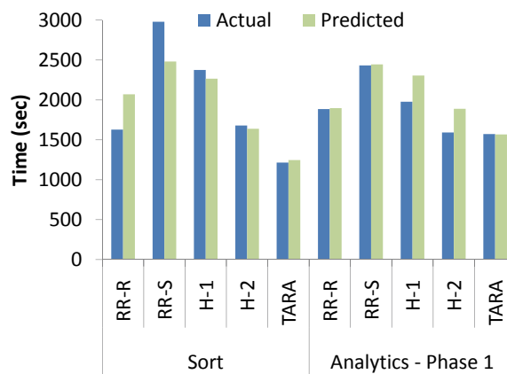
Figure 3: Benchmark Results
