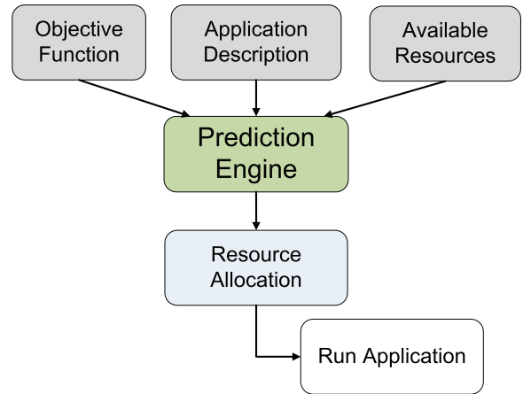
Figure 1: TARA’s Architecture
