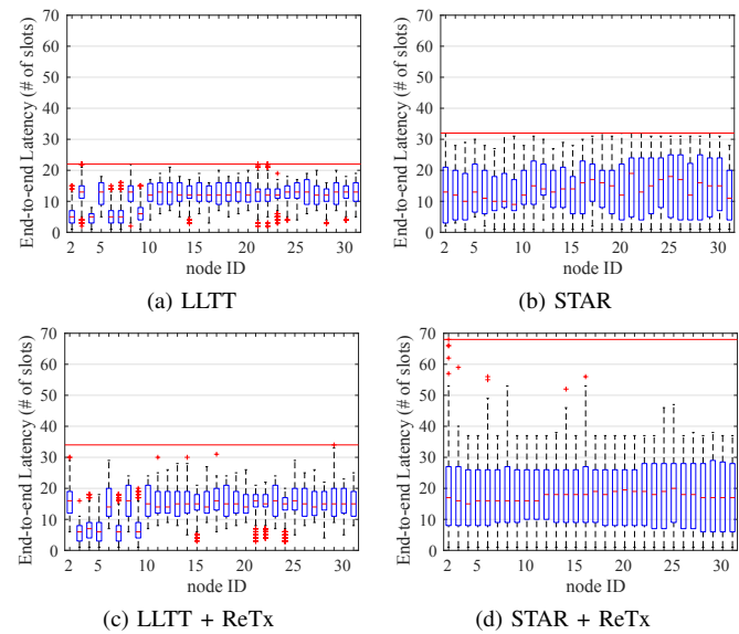
Fig. 8. End-to-end latency distribution of each node's communication towards the sink node. X-axes show the node number and the red lines show the maximum observed packet delivery latency for all nodes.
