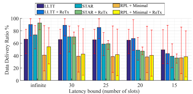
Fig. 9. Average DDR for different latency bounds, in presence of controlled interference on 4 out of 16 channels.
