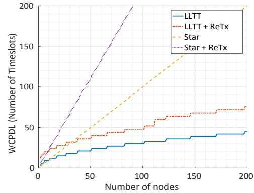
Fig. 5. Analytical worst case packet delivery latency vs the number of nodes in the network for TSCH schedules of star and LLTT topologies.
