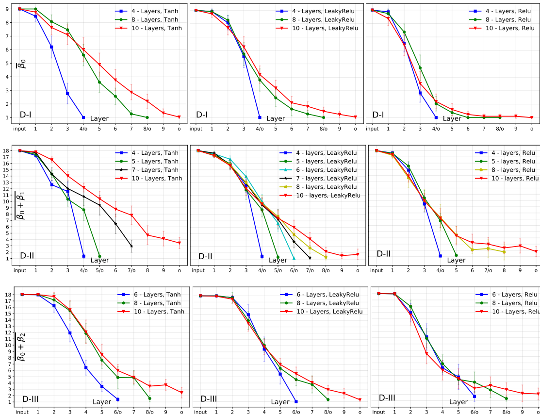
Figure 15: Mean values of topological complexity \omega(v_j(M_a)) , j = 0, 1, \dots, l , for fifteen-neuron-wide networks of varying depths. Error bars indicate \pm half standard deviation about the mean.
