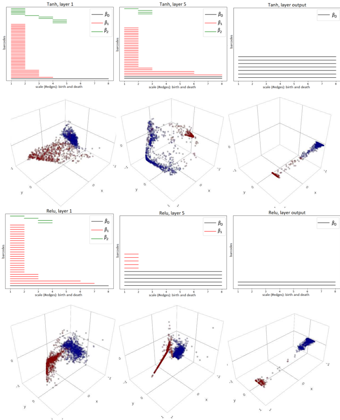
Figure 17: Persistence barcodes for neural networks trained on HTRU2 show topology changes in the ‘pulsar manifold’ M_a as it passes through the layers, activated with tanh ( top ) and ReLU ( bottom ). Scatter plots show principal component projections of M_a (red) and the ‘non-pulsar manifold’ M_b (blue) at the corresponding layers.
