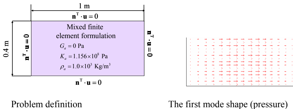
(b) Mixed finite element formulation without the elastic foundation
