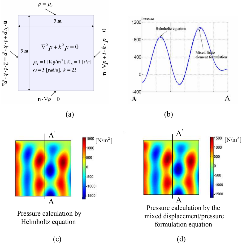
Figure 3. Analysis example 1: Acoustic domain analysis with the mixed formulation with various boundary conditions. (a) Problem definition (where p_0 = 123 Pa, and p_{in} = 1000 Pa), (b) the pressure distribution along AA', (c) the pressure distribution with the Helmholtz equation, and (d) the pressure distribution with the mixed finite element method.
