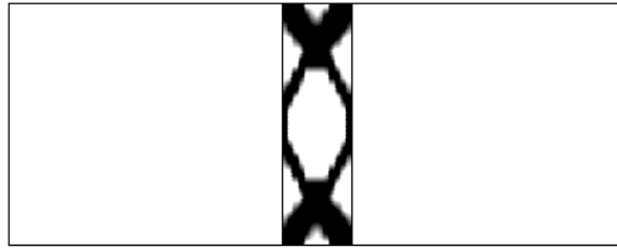
(a) \phi_{optimized} = 61.384 N (Mass=50.00%)
