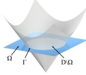
FIG. 4. Representation of a 2D geometry with a 3D level set function
