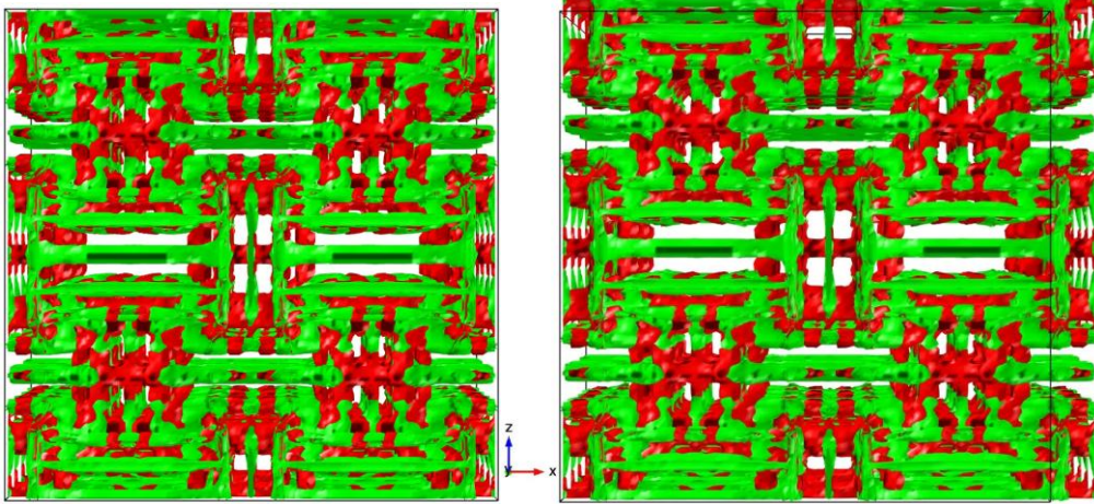
FIG. 23. Numerical verification of the 2 nd example of 3D multi-material NPR structure (xz-plane): (a) before (left) and (b) after (right) a displacement is applied in x direction.
