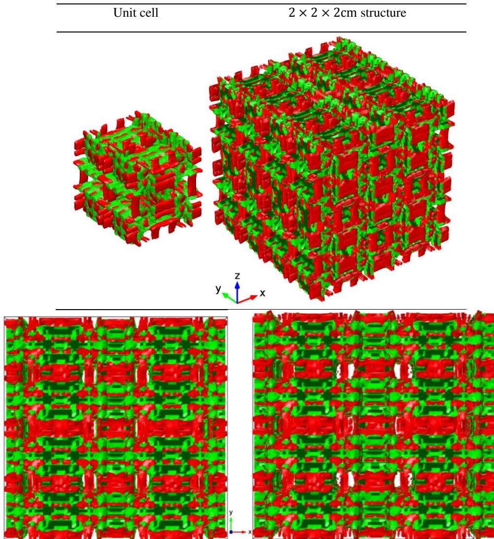
FIG. 19. Numerical verification of the 1 st example of 3D multi-material NPR structure (xy-plane): (a) before (left) and (b) after (right) a displacement is applied in x direction.
