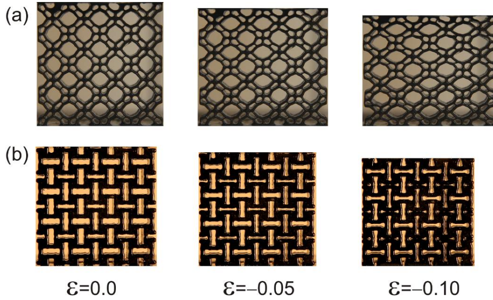
FIG. 14. Experimental images of the mechanical metamaterials at different levels of macroscopic strain: 0, -0.05, and -0.10. a) Specimen 1 with positive Poisson's ratio. b) Specimen 3 with negative Poisson's ratio.
