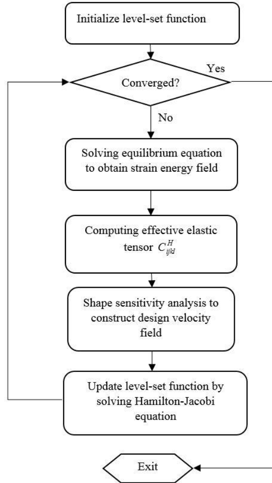
FIG. 6. Optimization flowchart
