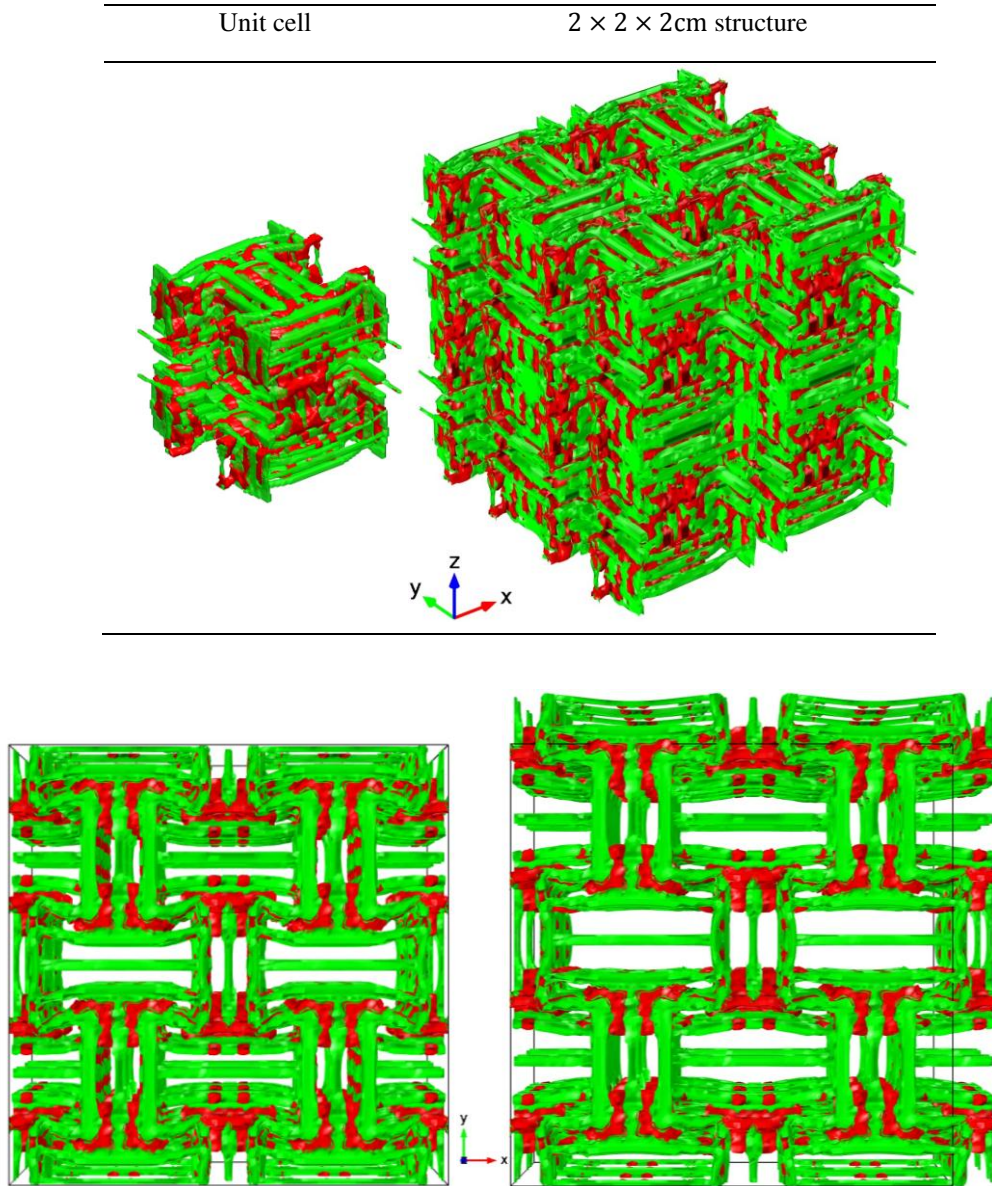
FIG. 22. Numerical verification of the 2 nd 3D multi-material NPR structure (xy-plane): (a) before (left) and (b) after (right) a displacement is applied in x direction.
