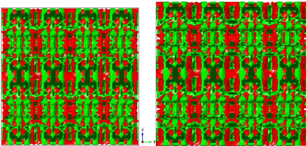
FIG. 21. Numerical verification of the 1 st example of 3D multi-material NPR structure (yz-plane): (a) before (left) and (b) after (right) a displacement is applied in y direction.
