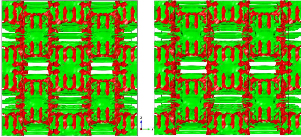
FIG. 24. Numerical verification of the 2 nd example of 3D multi-material NPR structure (yz-plane): (a) before (left) and (b) after (right) a displacement is applied in y direction.
