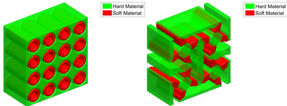
FIG. 10. The (a) Initial and (b) Final design of a 2D NPR metamaterial
