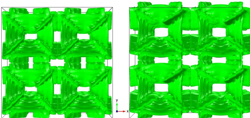
FIG. 18. Numerical verification of 3D NPR structure (xy-plane): (a) before (left) and (b) after (right) a displacement is applied in x direction.
