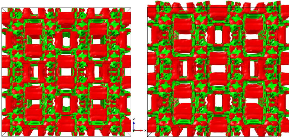
FIG. 20. Numerical verification of the 1 st example of 3D multi-material NPR structure (xz-plane): (a) before (left) and (b) after (right) a displacement is applied in x direction.
