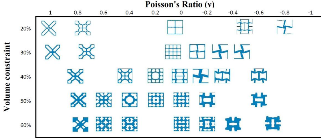
FIG. 9. Optimized auxetic metamaterials with various volume fractions and Poisson's ratios
