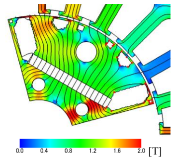
Fig.12 Smoothing of material boundaries
