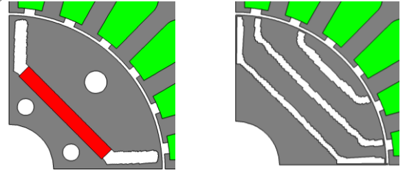
(b) Base model of IPM represented by \phi (c) Base model of SynRM represented by \phi Fig.4 IPM motor and base models represented by Gaussian bases
