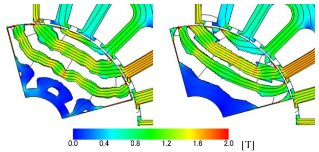
(a) Gaussian basis function (b) Polygon morphing Fig.10 Magnetic induction and flux lines in optimized SynRM
