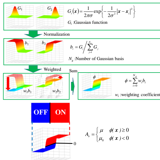
Fig.1 On/off method using normalized Gaussians
