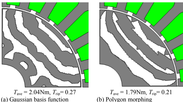
(a) Gaussian basis function (b) Polygon morphing Fig.9 Optimized shapes of SynRM
