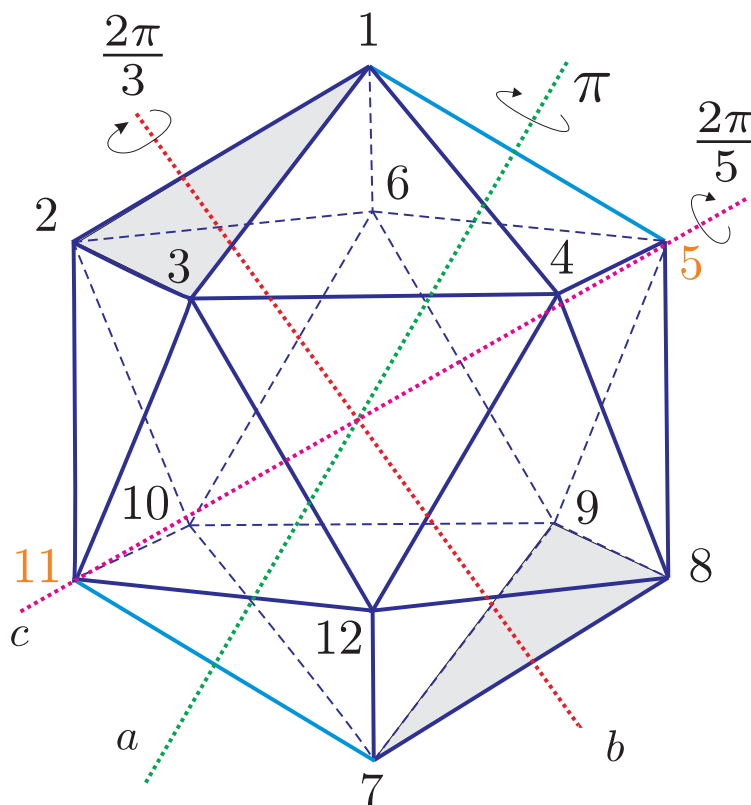
Figure 1: The icosahedron
