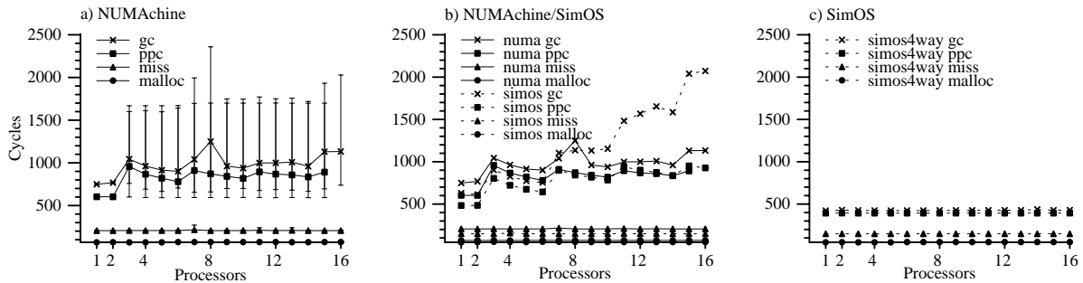
Figure 8: Nanobenchmarks: Garbage collection (gc), Protected Procedure Calls (ppc), in-core page miss handling (miss), and dynamic memory allocation (malloc), run under Tornado on NUMAchine (numa) and under Tornado on SimOS (simos). The left figure (a) shows the average number of cycles required on NUMAchine for n threads with range bars indicating the range over all threads. The middle figure (b) shows the average cycles required on NUMAchine and SimOS. The right figure (c) shows the average cycles required on SimOS configured with 4-way set associative caches.
