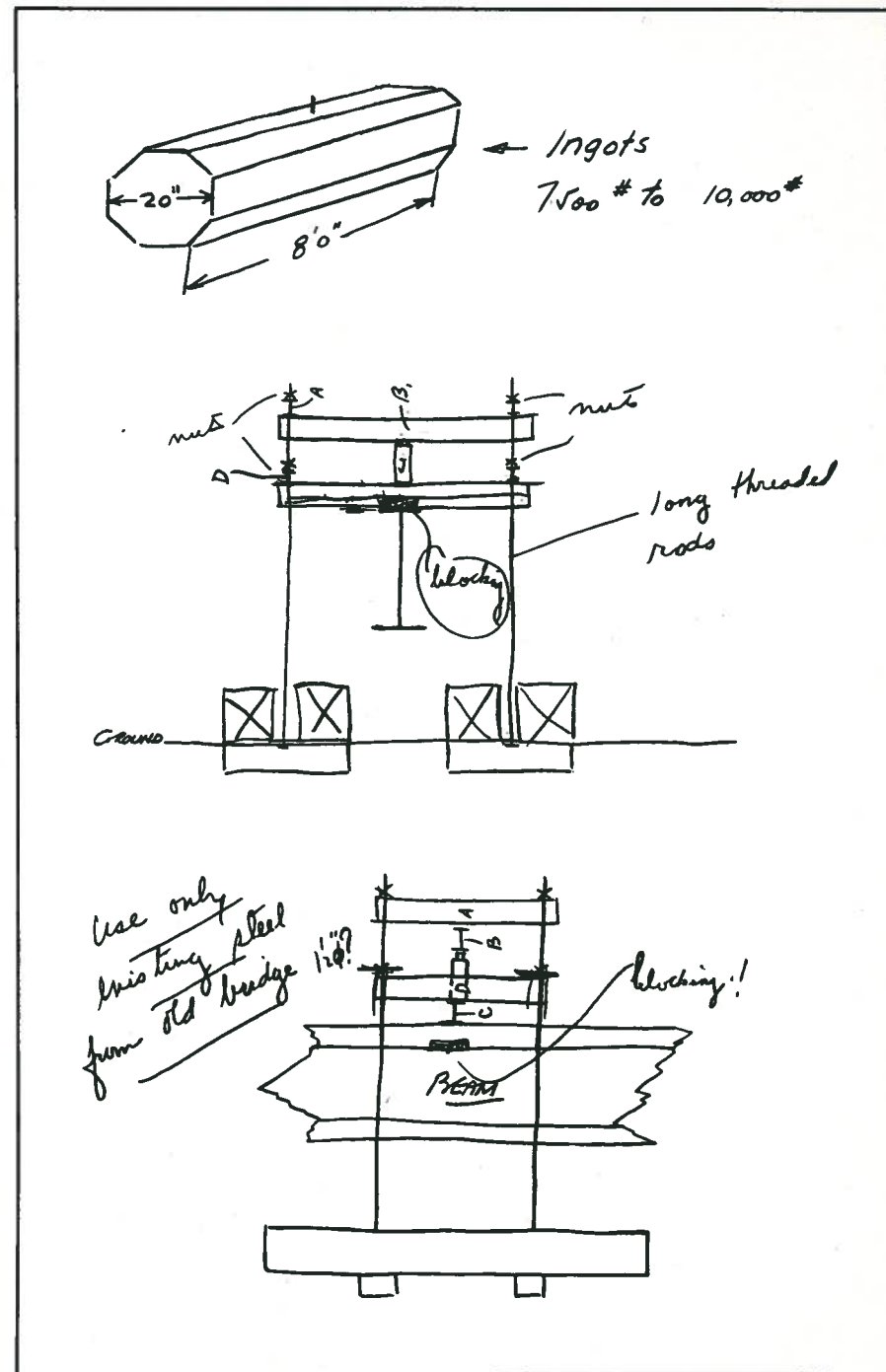
Fig. 10. Portions of Magnel's original rough sketches of the proposed testing arrangement for a 160-ft (49 m) girder used in the main span of the Walnut Lane Bridge. For contrast refer to the actual drawings (see Fig. 15).
