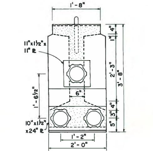
ROEBLING METHOD
