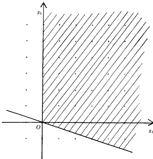
FIGURE 1. The region of \pi^\vee when n = 3
