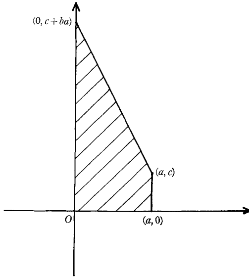
FIGURE 2. The polygon P_{a,b,c}
