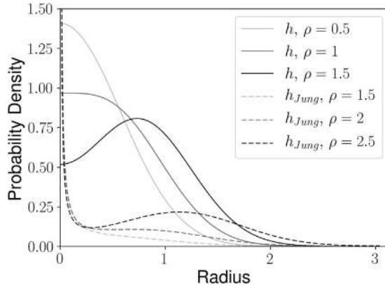
FIG. 6. The probability densities for \sigma = 0.5 along the geodesic \gamma in \mathbb{S}^d from (6) for our h (invariant under d ) and the h_{\text{Jung}} (for d = 2 ) distribution. Displaying a value for \rho below the respective boundary, at the boundary and above the boundary; namely, \rho = 1 for our h and \rho = 2 for the h_{\text{Jung}} distribution.
