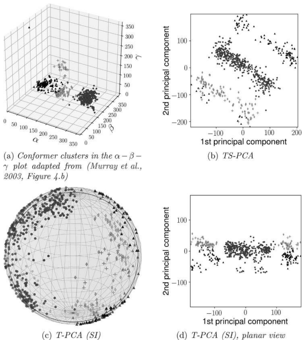
FIG. 9. Residues with C2'-endo sugar pucker with clustering following Murray et al. (2003). Three-dimensional heminucleotide angles (a); two-dimensional TS-PCA (b) approximation; two-dimensional T-PCA (SI) approximation, the small circle gives the 1D approximation (c); two-dimensional T-PCA (SI) approximation in planar representation (d).
