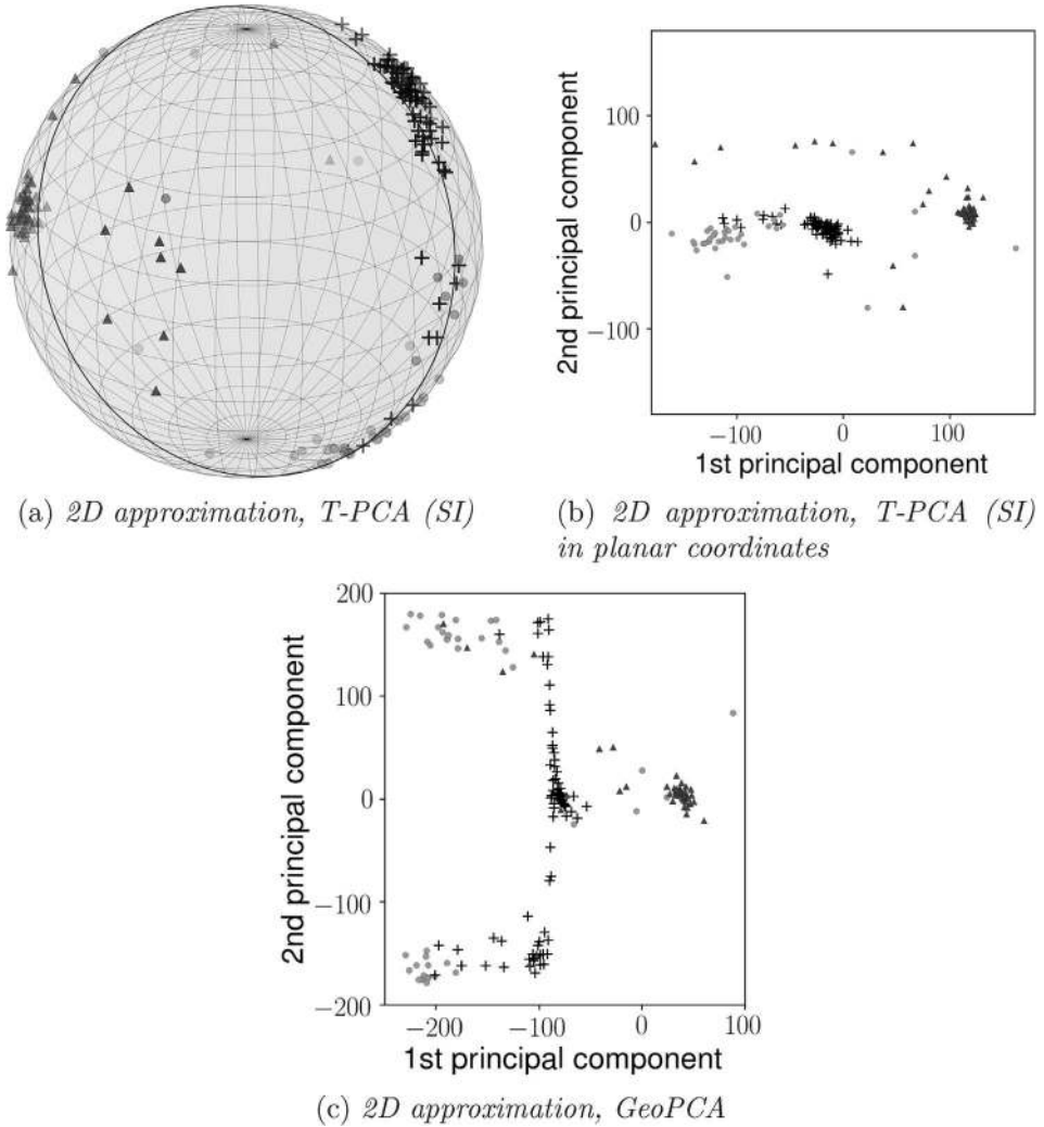
FIG. 8. Two-dimensional PCA approximations of the benchmark data set via T-PCA with SI ordering in natural spherical coordinates (a), in planar coordinates (b) and GeoPCA adapted from Sargsyan, Wright and Lim (2012), Figure 6, (c). The symbols represent the same clusters as in Figure 7.
