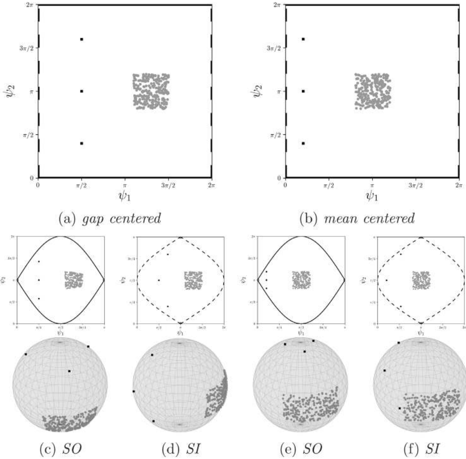
FIG. 5. All possibilities for gluing for T^2 , illustrated by a data set uniform in a square with three outliers. Using mean centered (b), the square is near the equatorial great circle [ \psi_1 = \pi for SO (e) and \psi_2 = \pi for SI (f)], and thus the square suffers little distortion, in comparison to the outliers. For gap centered (a), the outliers are less distorted, and for SO (c) the square is particularly distorted because the equatorial great circle ( \psi_1 = \pi ) is then between outliers and square. In both cases, SO decreases the spread of the outliers, SI increases it, more drastically for mean centered. Due to the torus' periodicity, lines of same type in the flat torus angle plots [top row, (a) and (b)] are identified. The respective outer angle is halved, the respective inner angle is unscaled [middle row, (c) and (d)]. Due to collapsing of some identified lines to points (the singularity set, in Figure 4 this is the circle along which the donut is cut), north and south pole of each sphere are identified [bottom row, (e) and (f)].
