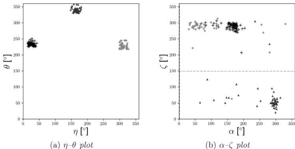
FIG. 7. (a) The benchmark data set of Sargsyan, Wright and Lim (2012) with their three preselected clusters in the \eta - \theta plot. (b) The benchmark data set plotted for the two most discriminant angles ( \alpha , \zeta ) chosen out of the seven dihedral angles; in the “donut to sausage” transformation along the dashed lines the corresponding angles are collapsed to a single point.
