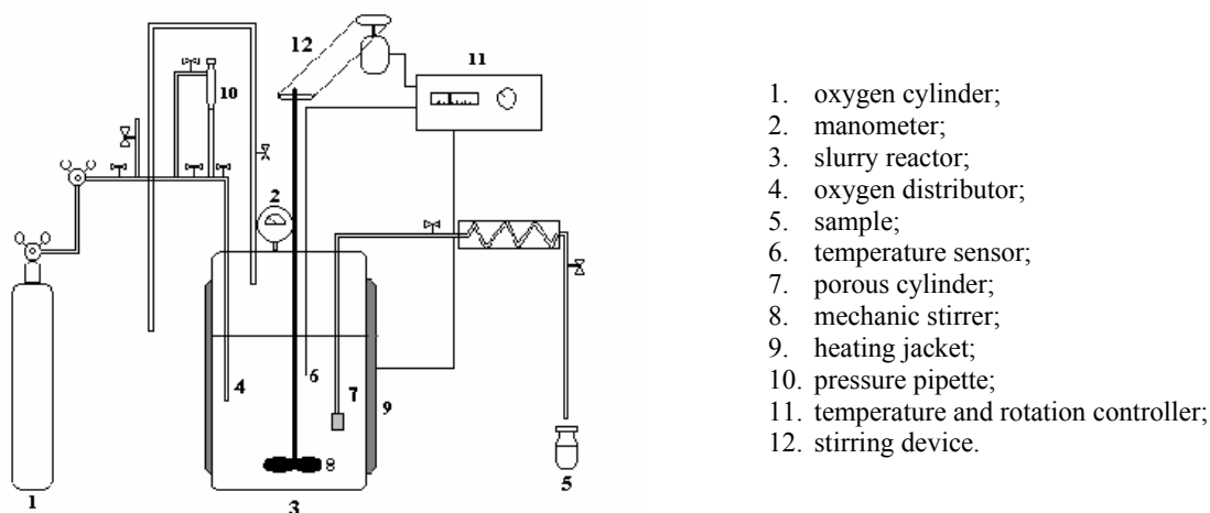
Figure 1: Experimental setup
