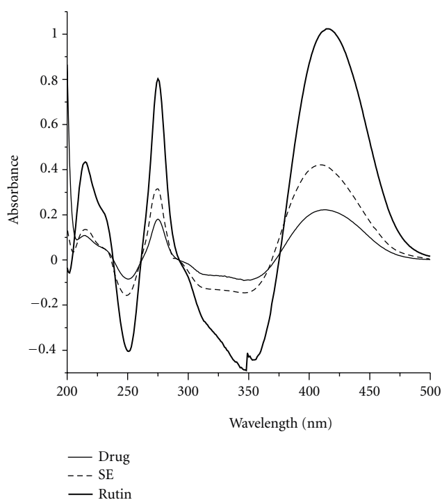
FIGURE 1: Spectrum for AlCl 3 -flavonoid complexes: herbal material (drug), aqueous extractive (SE) and standard (rutin).
