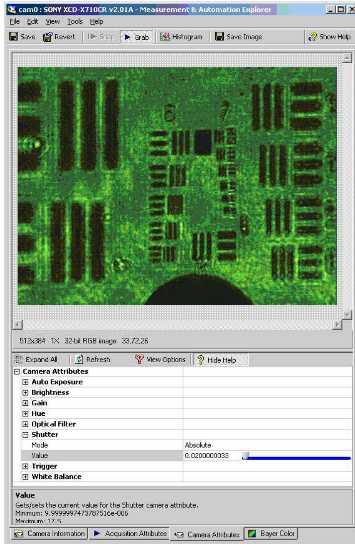
Figure 4.4 TIR camera MAX image of RT chip in glycerin on truncated SFL11 TIR prism; Groups 6 and 7. Tilt compression in phase image is in x-direction. Illumination is with green laser object beam. Shutter speed at 0.02s. Note bubble curvature at bottom FOV; black for loss of signal (LOS).
