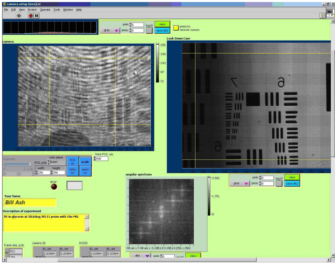
Figure 4.6. Camera Setup (iee).vi routine; Operators console. Hologram on left Lookdown camera feed on right. FOV calibrated at 430um. The power levels of the object and reference beam are too high, as evinced by the power bar top left and the angular spectrum diffraction products at bottom center, and are reduced either by adjusting the polarizers or increase of camera speed in MAX. This setup required further adjustment.
