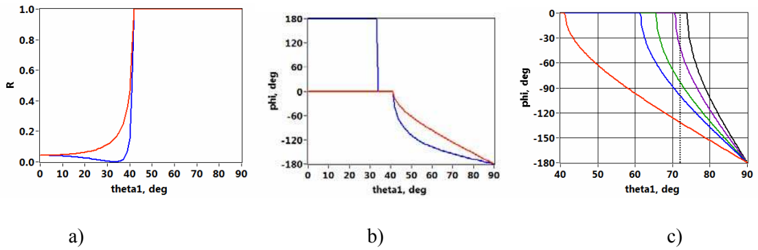
Fig. 2.2. a) Reflectance R and b) reflection phase, \phi ( \varphi in text) vs. angle of incidence, \theta_1 ( \theta_l in text) for the relative index, n_1/n_2 = 1.517 . [red: s-polarization; blue: p-polarization] c) Reflection phase of s-polarization vs. angle of incidence for various relative indices: n_1 = 1.517 ; n_2 = 1.000 (red), 1.333 (blue), 1.382 (green), 1.432 (purple), 1.458 (black).
