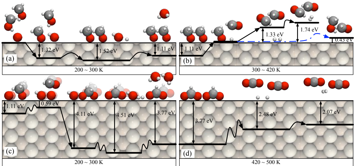
FIG. 5: The scenarios for the partial and the total oxidation of methanol on oxygen-covered Cu(110) with respect to the reference energy E_{\text{ref}} = nE[\text{O}/\text{Cu}(110)] + 2E[\text{CH}_3\text{OH}^{(g)}] . We assume that the oxygen atoms are initially located at the pseudo fcc hollow site within a p(2 \times 2) periodicity. The methoxy and formate formation schemes are illustrated in panels (a) and (c), respectively. Panel (b) describes the final steps in the partial oxidation of methanol from methoxy to formaldehyde while panel (d) shows the corresponding final steps in the total oxidation from formate to \text{CO}_2 operative at higher temperatures.
