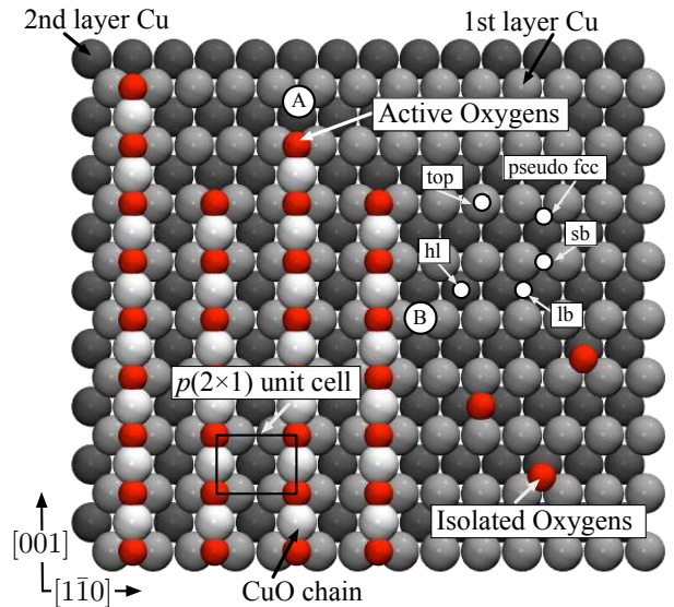
FIG. 1: Schematic presentation of the oxygen-covered Cu(110) surface. Oxygen induces a p(2 \times 1) added-row reconstruction consisting of CuO chains that form a stripe phase. The terminal oxygen species active for methanol oxidation are located at the [001] edge of the chains.
