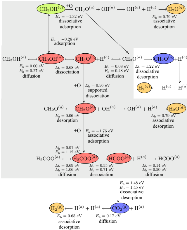
FIG. 4: Schematic diagram of methanol oxidation on oxygen-covered Cu(110). The shaded area represents the precursor reactions below 300 K for partial and total oxidations.
