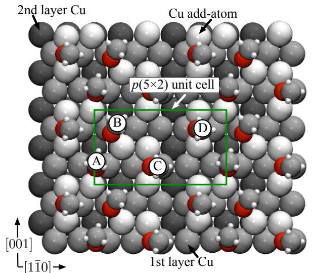
FIG. 3: Calculated p(5 \times 2) methoxy structure on Cu(110) based on structural models proposed by Leibsle et al. [11, 31].
