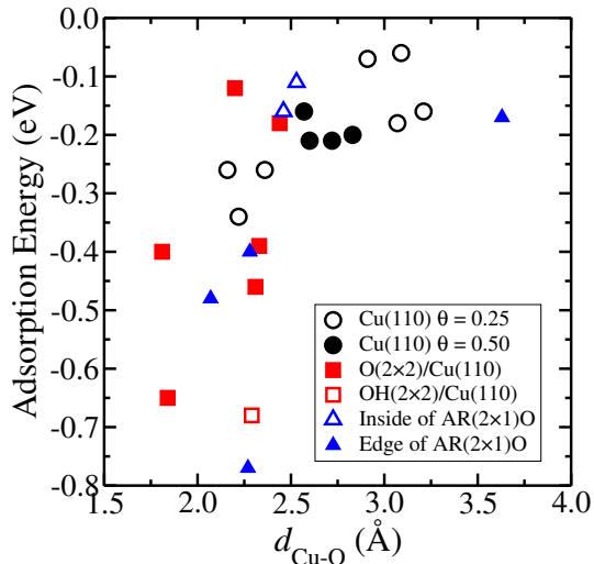
FIG. 2: Adsorption energy of methanol as a function of the distance between the methanol oxygen atom and the nearest Cu atom. The energies are defined with respect to the isolated substrate and methanol in the gas phase. The methanol coverage for the clean Cu(110) substrate is \theta_{\text{CH}_3\text{OH}} = 0.25 and 0.5, whereas it is 0.25 for the oxygen- and hydroxyl covered Cu(110) surface within a p(2 \times 2) geometry. For the added row reconstruction (AR), there is one methanol molecule in the corresponding unit cells that are described in section II.
