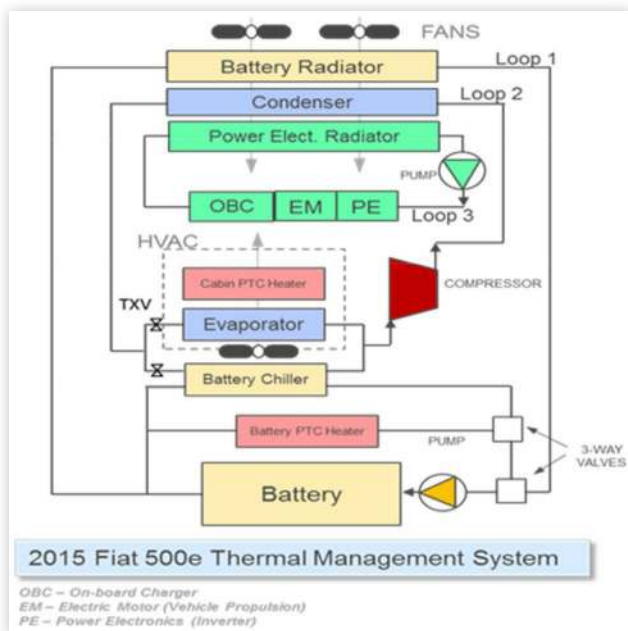
FIGURE 2 Three thermal sub-systems of Fiat 500e BEV
