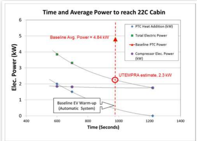
(a) Time to reach cabin set-point temperature of 22°C if different PTC heat is applied
