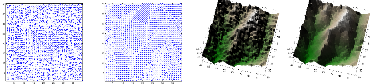
Figure 5. Optimization on the two-dimensional unit sphere applied to denoising of normals in S^2 for three-dimensional visualization. Left to right: Input normal field (two-dimensional top-projection) computed from noisy height map; result of Rudin-Osher-Fatemi denoising in S^2 ; height map with shading computed from unprocessed noisy normal field; height map with shading computed from denoised normal field. Similar to the scalar-valued case, the ROF model minimizer preserves discontinuities, e.g., along the ridges of the mountains.
