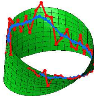
Figure 1. Denoising of a function with values in a manifold. We propose an algorithm for total variation (TV)-regularization of functions with values on arbitrary Riemannian manifolds. This example shows the TV-denoising ( blue ) of a one-dimensional function ( red ) u : [0, 1] \rightarrow \mathcal{M} with values in the Moebius band \mathcal{M} . Characteristic of TV-denoising is the reduction of contrast, which corresponds to the shrinking of the curve. The key idea is to represent the manifold by a set of grid points (labels) and to solve a convex optimization problem that admits sub-label accuracy : in the above example, the blue points may lie between grid-points.
