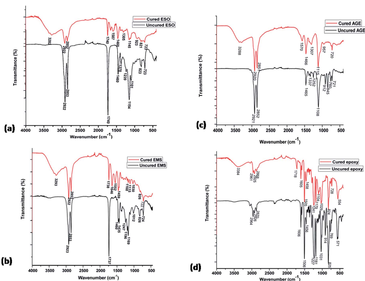
Fig. 3 FTIR spectra of crosslinked resin (a) ESO/TETA, (b) EMS/TETA, (c) AGE/TETA and (d) epoxy/TETA.
