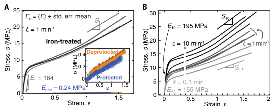
Fig. 3. Uniaxial tensile tests. (A) Engineering stress as a function of strain of protected (blue), deprotected (orange), and iron-treated samples (gray); strain rate, \dot{\epsilon} = 1 \text{ min}^{-1} . (B) Strain-rate dependency ( \dot{\epsilon} = 0.1, 1, \text{ and } 10 \text{ min}^{-1} ) of iron-treated samples.
