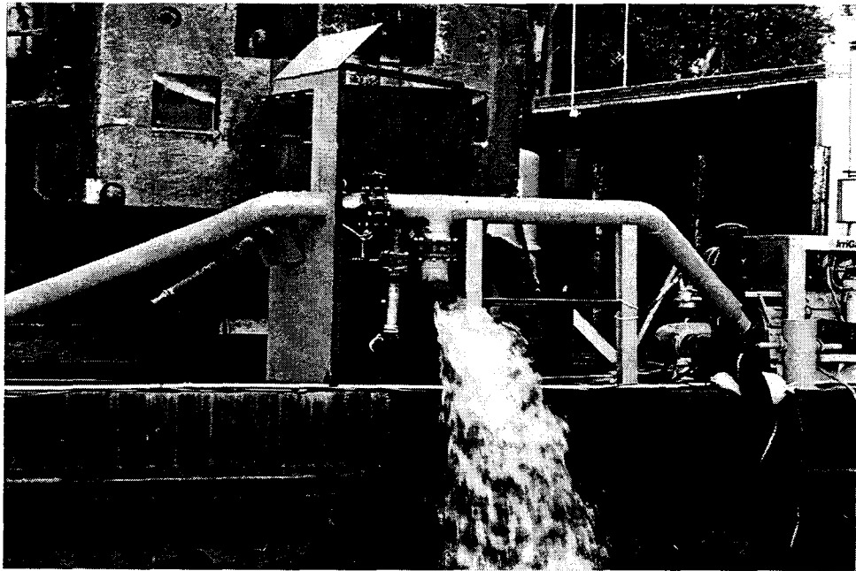
Figure 5. Fluidization valve-control system
