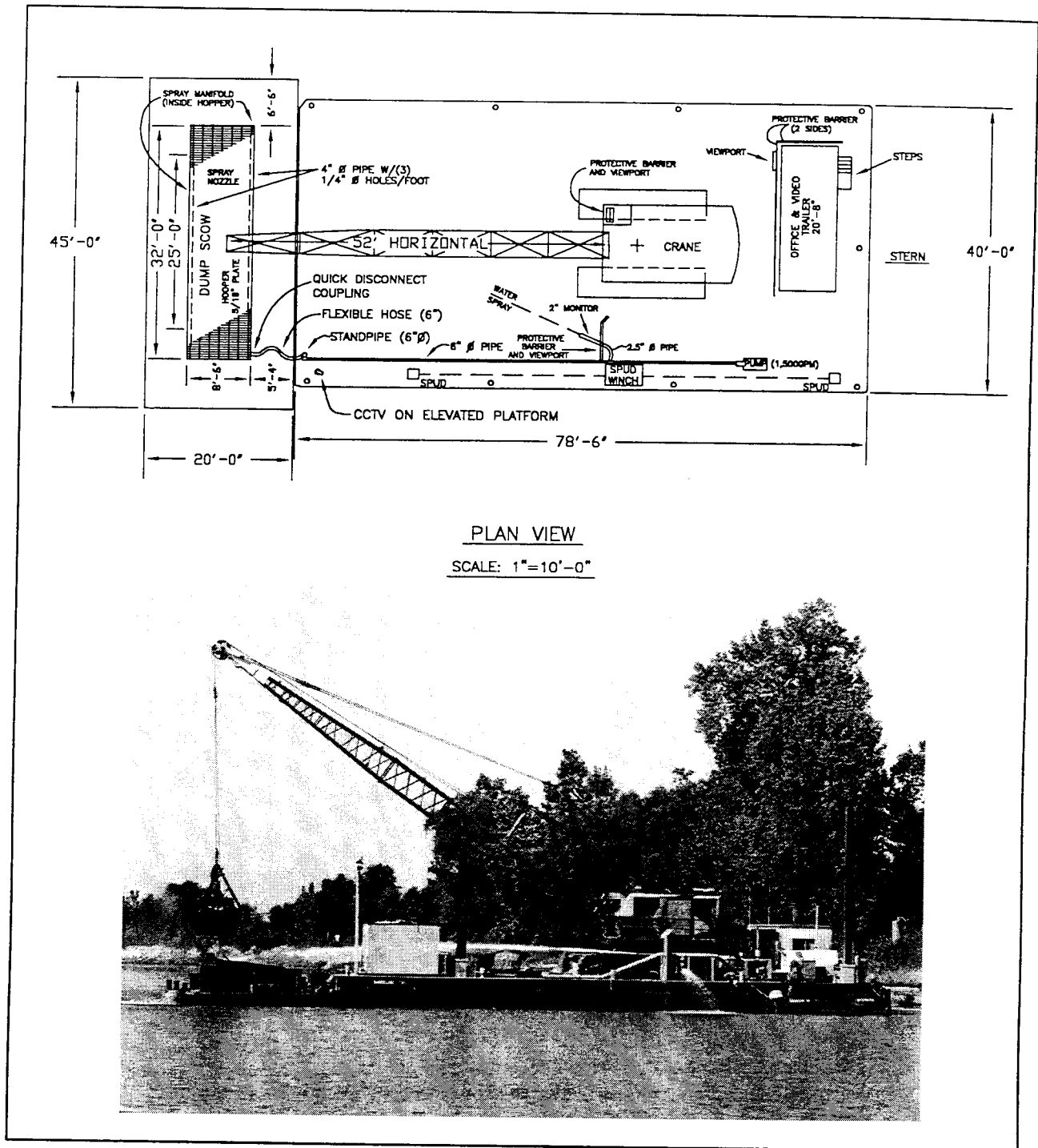
Figure 3. Deck layout (Courtesy of Shoreline Contractors, Inc.) and photograph of UXO dredging system
