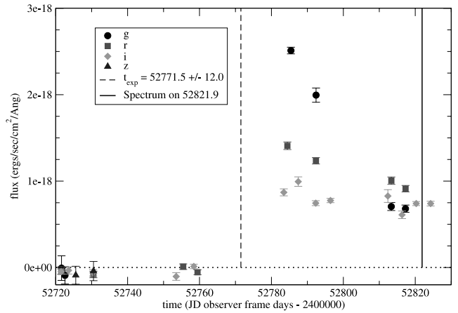
FIG. 6.—SNLS g'r'i'z' light curves (in f_{\lambda} ) for SNLS-03D3ce at z = 0.2881 . Unfortunately, this SN was not observed in z' on the plateau. At this redshift z' overlaps nicely with the rest-frame I band; thus, the V-I color had to be extrapolated from bluer colors than desired for this SN II-P. [See the electronic edition of the Journal for a color version of this figure.]
