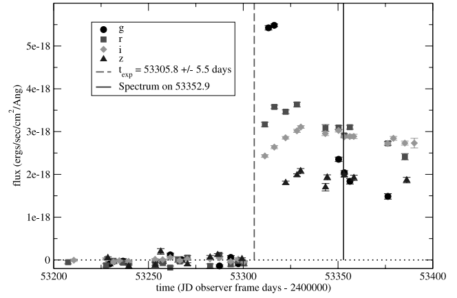
FIG. 9.—SNLS g'r'i'z' light curves (in f_{\lambda} ) for SNLS-04D1pj at z = 0.1556 . [See the electronic edition of the Journal for a color version of this figure.]
