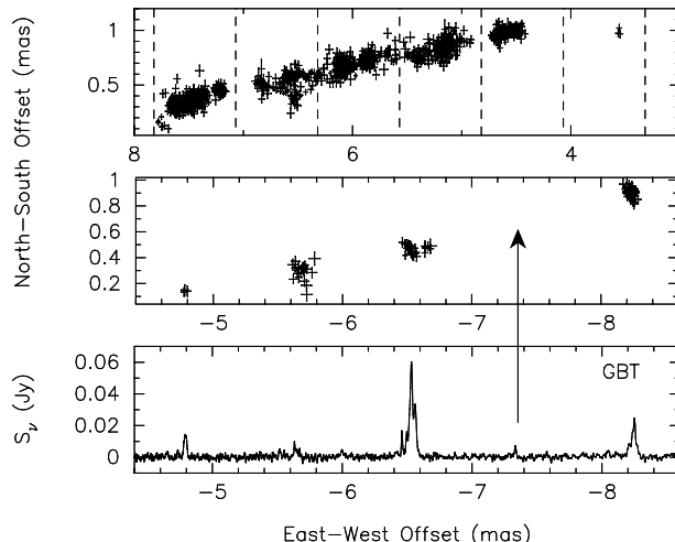
FIG. 17.— Top : Sky positions of redshifted high-velocity emission in the NGC 4258 disk obtained using VLBI over 18 epochs. Dashed lines mark nodes at characteristic wavelengths of 0.75 \text{ mas} , proposed by Maoz (1995). Middle : Blueshifted components in the NGC 4258 disk. Bottom : GBT spectrum of the blueshifted high-velocity emission taken on 2003 October 23. Velocity has been represented as approximate east-west offset. The arrow marks the velocity of the “missing” blue component predicted by the Fourier analysis and detected independently in the spectrum.
