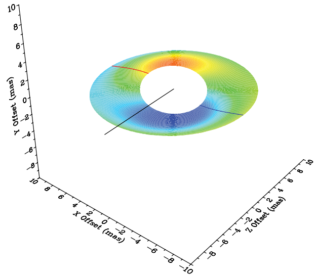
FIG. 10.—Best-fitting maser disk from Herrnstein et al. (2005) viewed from [-40, 40, -50] . The LOS is shown as a line extending beyond the outer edge of the disk in black along the z -direction. Solid color contours show disk elevation, where red is the maximum and dark blue is the minimum. The disk midline for \phi = 0^\circ and 180^\circ is shown for redshifted emission ( red line ) and blueshifted emission ( blue line ), respectively. Low-velocity (systemic) masers lie in the concavity on the front side of the disk.
