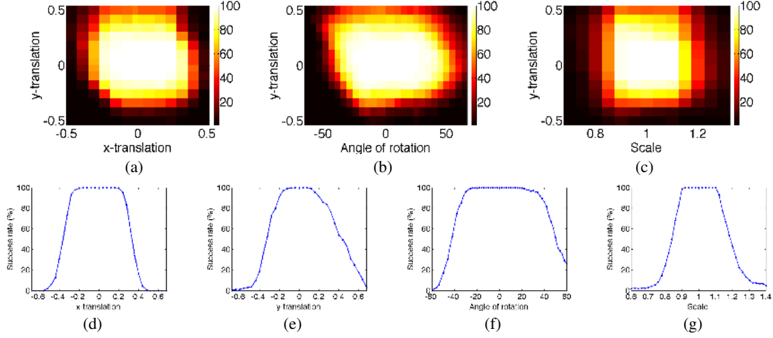
Fig. 3. Region of attraction. Fraction of subjects for which the algorithm successfully aligns a synthetically perturbed test image. The amount of translation is expressed as a fraction of the distance between the outer eye corners, and the amount of in-plane rotation in degrees. Top row: (a) Simultaneous translation in x and y directions. (b) Simultaneous translation in y direction and in-plane rotation. (c) Simultaneous translation in y direction and scale variation. Bottom row: (d) Translation in x direction only. (e) Translation in y direction only. (f) In-plane rotation only. (g) Scale variation only.
