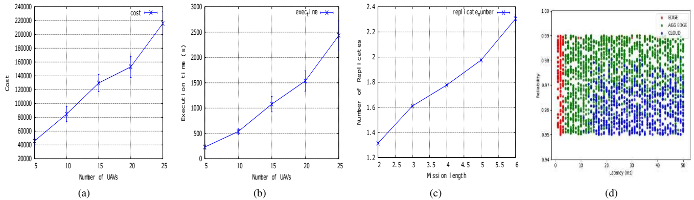
Fig. 3: Performances evaluation.
