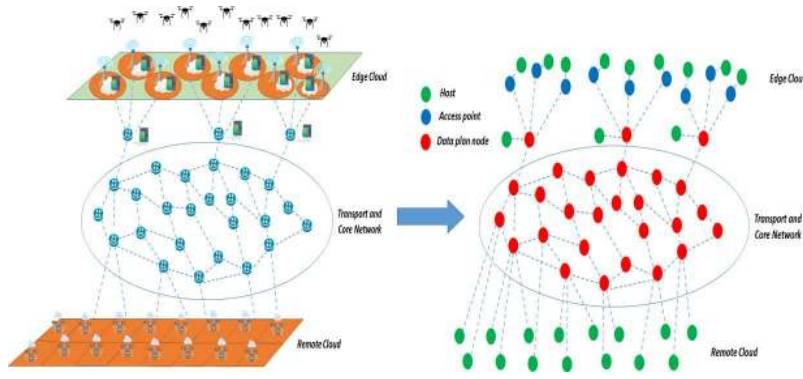
Fig. 2: Network Model.
