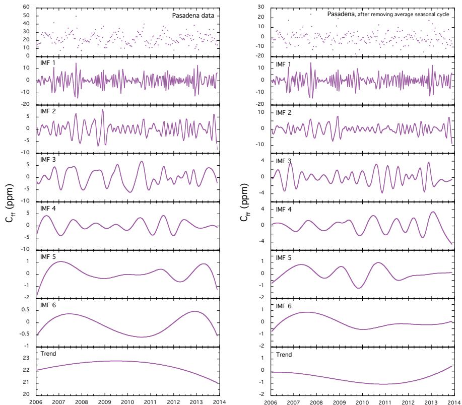
Figure C1. Time series of all of the results from the ensemble empirical mode decomposition (EEMD) analysis of the Pasadena C ff . The left set of panels shows the results for the raw data, whereas the right column shows those for the data after subtraction of the average seasonal cycle. The long-term trend reflecting the economic downturn of the Great Recession is reflected clearly in IMF 6 and the trend of the data after the pronounced seasonality is removed (right-hand column), although there is some evidence of it in IMF 6 of the raw C ff data.
