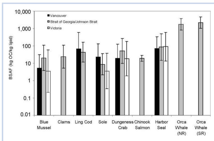
Figure 3. Log BSAF (kg OC/kg lipid) of \Sigma PCB for different wildlife species at 3 locations in the Pacific North west of North America, i.e., Vancouver Harbor (black), Strait of Georgia (gray), and Victoria Harbor (white). Error bars present standard deviations of the geometric mean.
