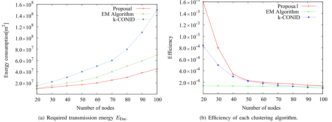
Fig. 4. Energy consumption for data transmission and efficiency.
