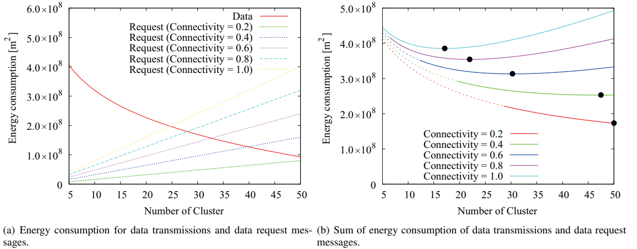
Fig. 5. Effect of the number of cluster.
