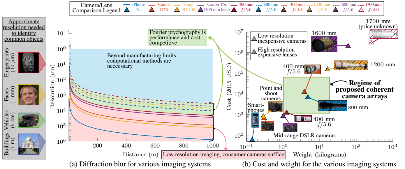
Fig. 2. Diffraction blur limits in long distance imaging. (a) Diffraction blur spot size as a function of distance for common and exotic imaging systems. Consumer cameras (shaded in the pink region) are designed for close to medium range imaging but cannot resolve small features over great distances. Professional lenses (green region) offer improved resolution but are bulky and expensive. Identifying faces 1 kilometer away is possible only with the most advanced super telephoto lenses, which are extremely rare and cost upwards of $2 million US dollars [49]. Obtaining even finer resolution (blue region) is beyond the capabilities of modern manufacturing; the only hope for obtaining such resolution is to use computational techniques such as Fourier ptychography. (b) Affordable camera systems (solid marks) are lightweight but cannot resolve fine details over great distances as well as professional lenses (striped marks) which are heavy and expensive. We propose using a camera array with affordable lenses and active lighting to achieve and surpass the capabilities of professional lenses. Note: These plots only account for diffraction blur and do not consider other factors limiting resolution (see TABLE I for more details).
