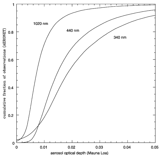
FIG. 6.—Aerosol optical depth statistics. Cumulative distributions of aerosol optical depth on Mauna Loa are shown from the AERONET observations over the period shown in Fig. 2.
