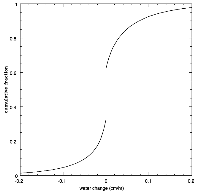
FIG. 11.—Cumulative plot of rate of change of AERONET's derived precipitable water content (centimeters per hour). For a typical value of 0.2 cm this implies that measurements more frequently than hourly are required to track 10% changes with confidence.
