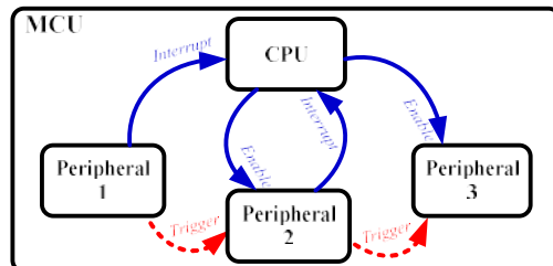
Fig. 1. Peripherals interaction in a centralized (blue solid line) and decentralized (red dashed line) architecture.
