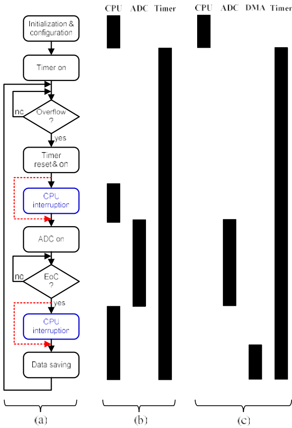
Fig. 2. (a) Flowchart of the measurement process; differences between ISR and PTP techniques are highlighted in blue solid line and red dashed line, respectively. Time intervals in which the embedded resources are activated when applying the (b) ISR, and (c) PTP techniques.
