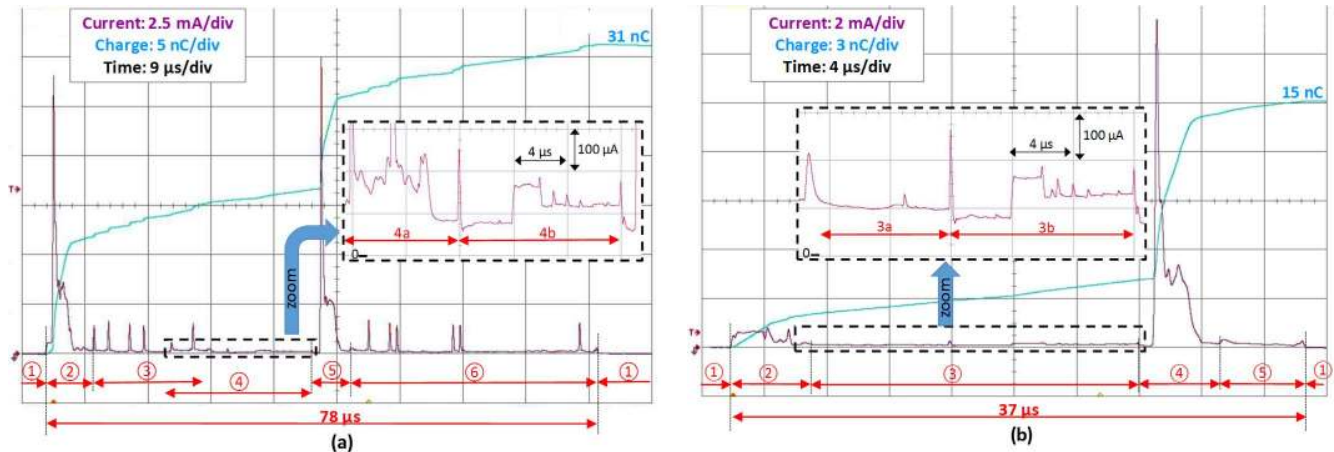
Fig. 4. Profile of the current consumption and the resulting charge—obtained by integrating the former—when the MCU applied (a) the ISR-based approach represented in Fig. 2(b), and (b) the PTP approach represented in Fig. 2(c).
