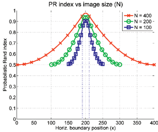
Fig. 3. Plot of PR index computed using (4) for the scenario of Fig. 2 with fixed w = 20 and varying image size N . Note that the function profile is maintained while the maximum attainable PR index increases with N .
