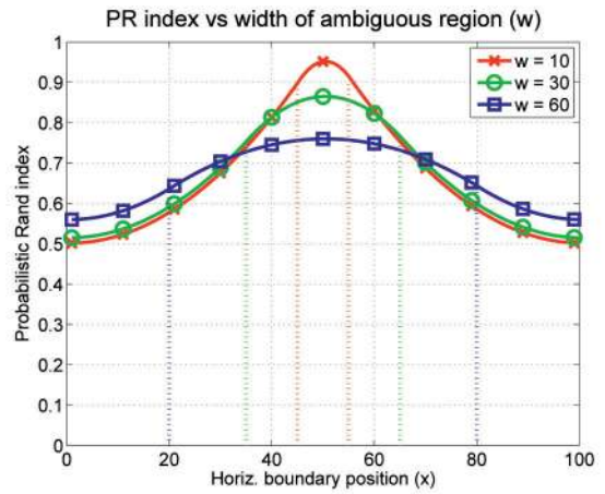
Fig. 4. Plot of PR index computed using (4) for the scenario of Fig. 2 with fixed image size ( N = 100 ) and varying w . Note that the function is everywhere continuous, concave in the zone of ambiguity, and convex elsewhere.
