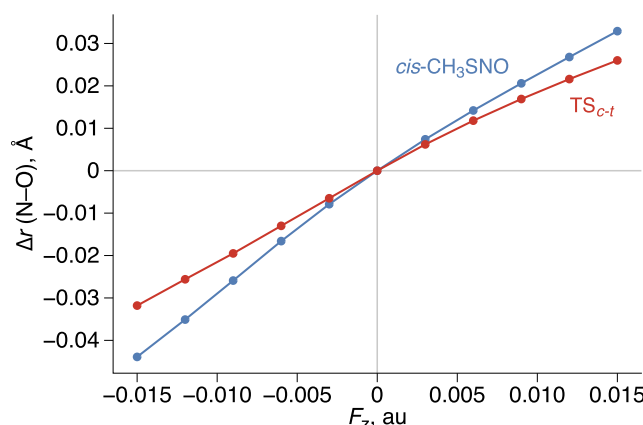
FIG. 5. EEF effect on the N—O bond lengths in cis - \text{CH}_3\text{SNO} and \text{TS}_{c-t} , calculated with CCSD(T)-F12/VDZ-F12 methods.
