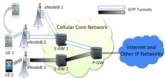
Fig. 1. LTE data plane
