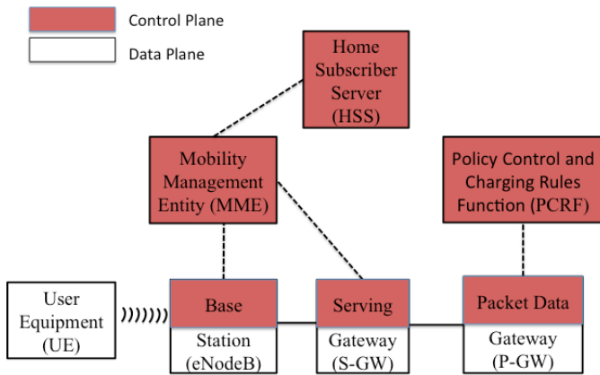
Fig. 2. Simplified LTE network architecture
