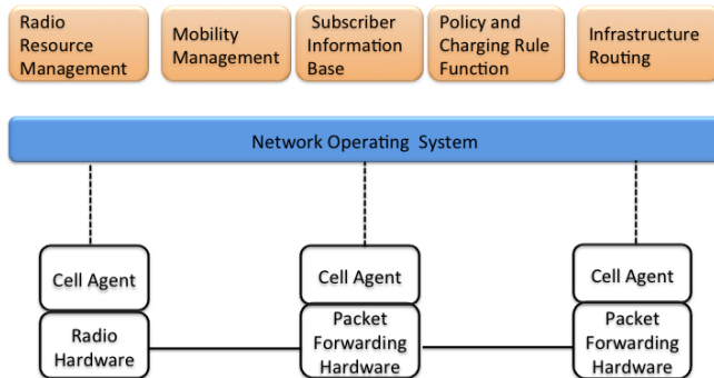
Fig. 3. Cellular SDN architecture
