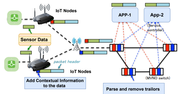
FIGURE 20. Context-aware SDN NFV based IoT architecture.
