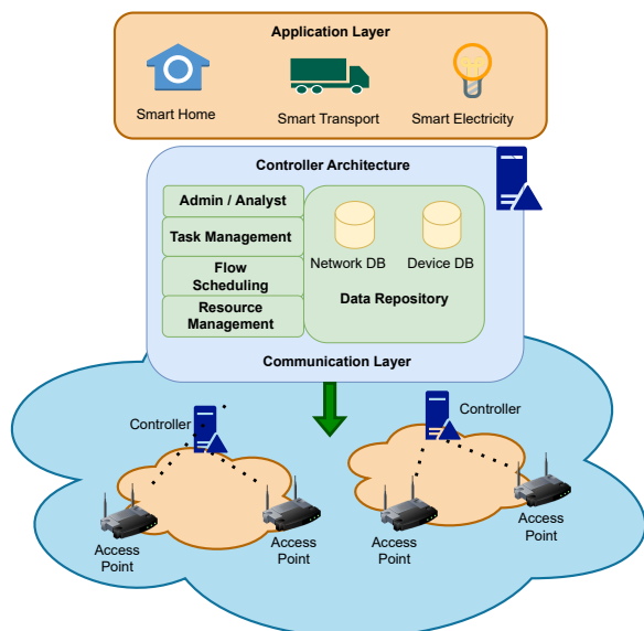
FIGURE 26. UbiFlow system architecture.
