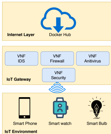
FIGURE 17. NETRA: Enhancing IoT Security using NFV.
