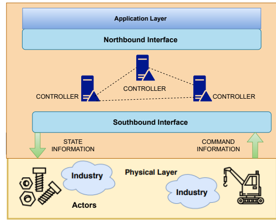
FIGURE 28. A WSAN framework based on SDN application.
