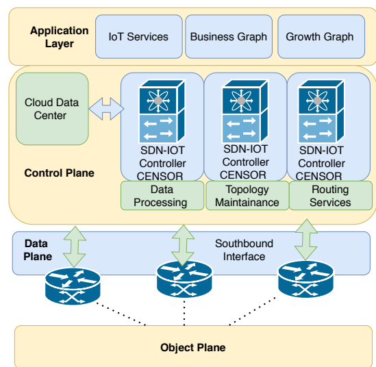
FIGURE 30. CENSOR: Cloud-enabled secure IoT architecture over SDN paradigm.
