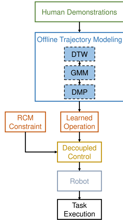
Fig. 4. Developed control framework. After multiple demonstrations, the demonstrated motion curves are aligned with DTW, and GMM is introduced to extract the similarity of the DMP for the manipulation task. A learned manipulation curve is obtained from the trained model. Finally, the learned operation is performed with the decoupled controller respecting the RCM constraint.
