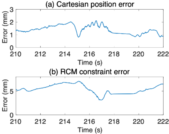
Fig. 13. Online performance for performing the learned trajectory
