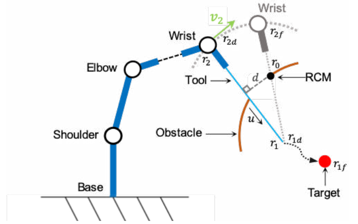
Fig. 2. RCM constraint control: a null-space kinematic controller is utilized to achieve the RCM constraint. As it is shown in the above picture, d is the RCM constraint error, calculated by the distance between the trocar position ( r_0 ) and the tool shaft. The tool-tip is controlled to reach the target from the actual position ( r_1 ) in the patient's abdominal cavity, and v_2 is the desired velocity to drive the wrist to the desired position ( r_{2d} ) until it reaches ( r_{2f} ).
