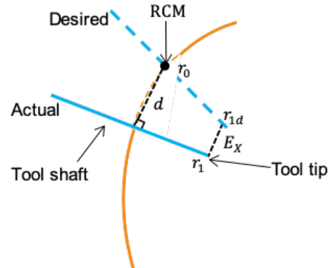
Fig. 12. Performance measurement. d is the RCM constraint error and E_x is the Cartesian error on the tool tip. The “Actual” link means the actual tool shaft placement while the “Desired” link represents its corresponding desired placement.
