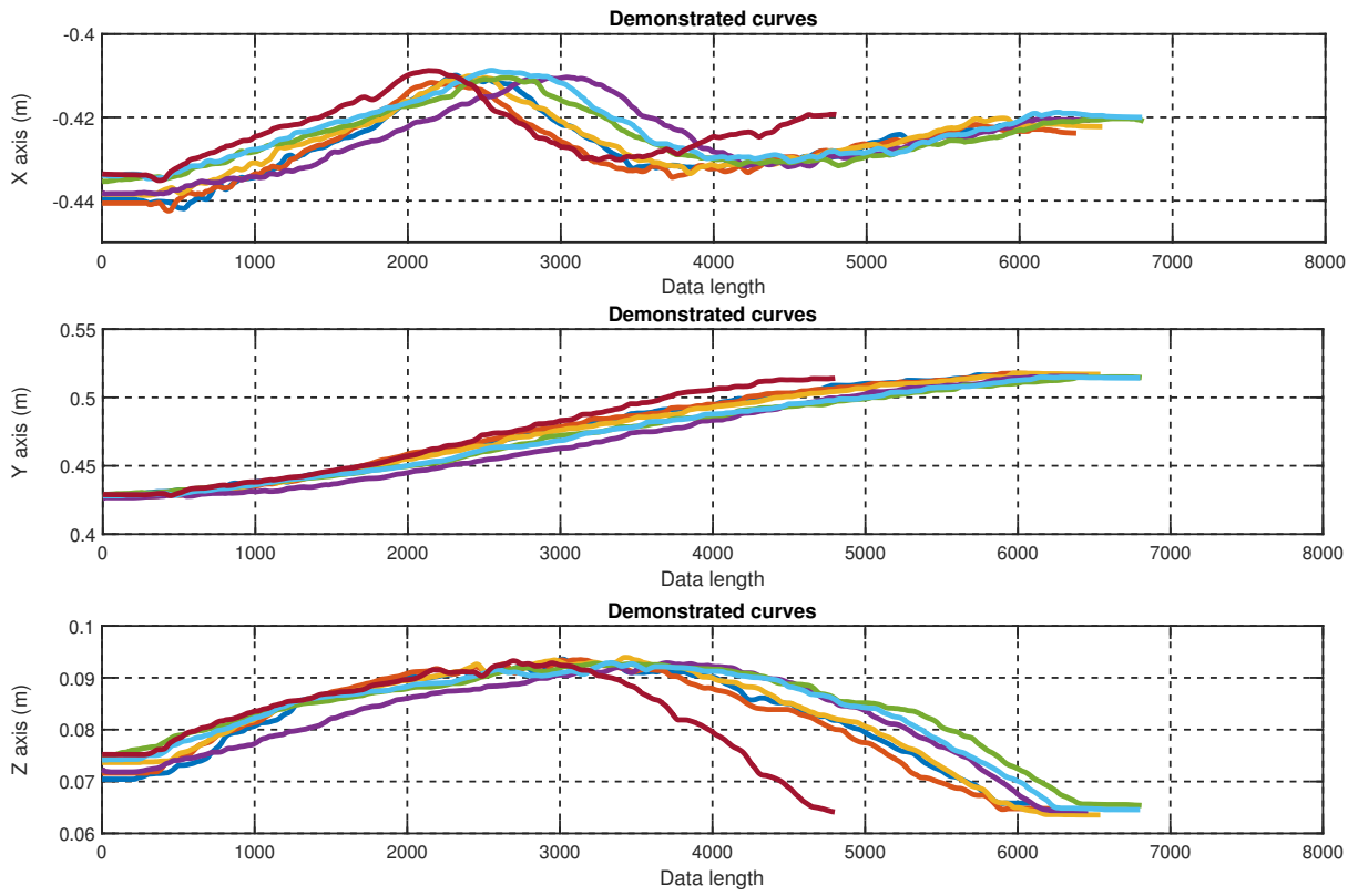
Fig. 8. Demonstrated operation curves in 3-axis. The demonstrated data lengths are different due to the difference of the operation time.
