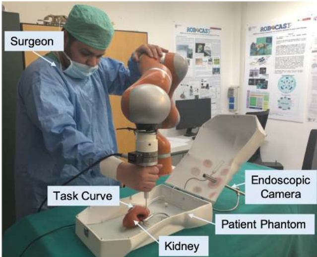
Fig. 5. Demonstration setup scene in open surgery. A kidney tissue model with a size of around 135 \times 45 \times 30mm^3 is presented in the 3-D patient phantom ( 170 \times 210 \times 100mm^3 ). The patient phantom is opened, and a metal clip fixes the kidney model in the abdominal cavity. A white task curve is drawn in advance along a blood vessel on the surface of the kidney to serve as the specific tracking task. The robot is activated in hands-on control mode to enable the surgeon to relocate the surgical tip by hand. The “surgeon” is commanded to do multiple demonstrations of tracking the white task curve with the surgical tip.
