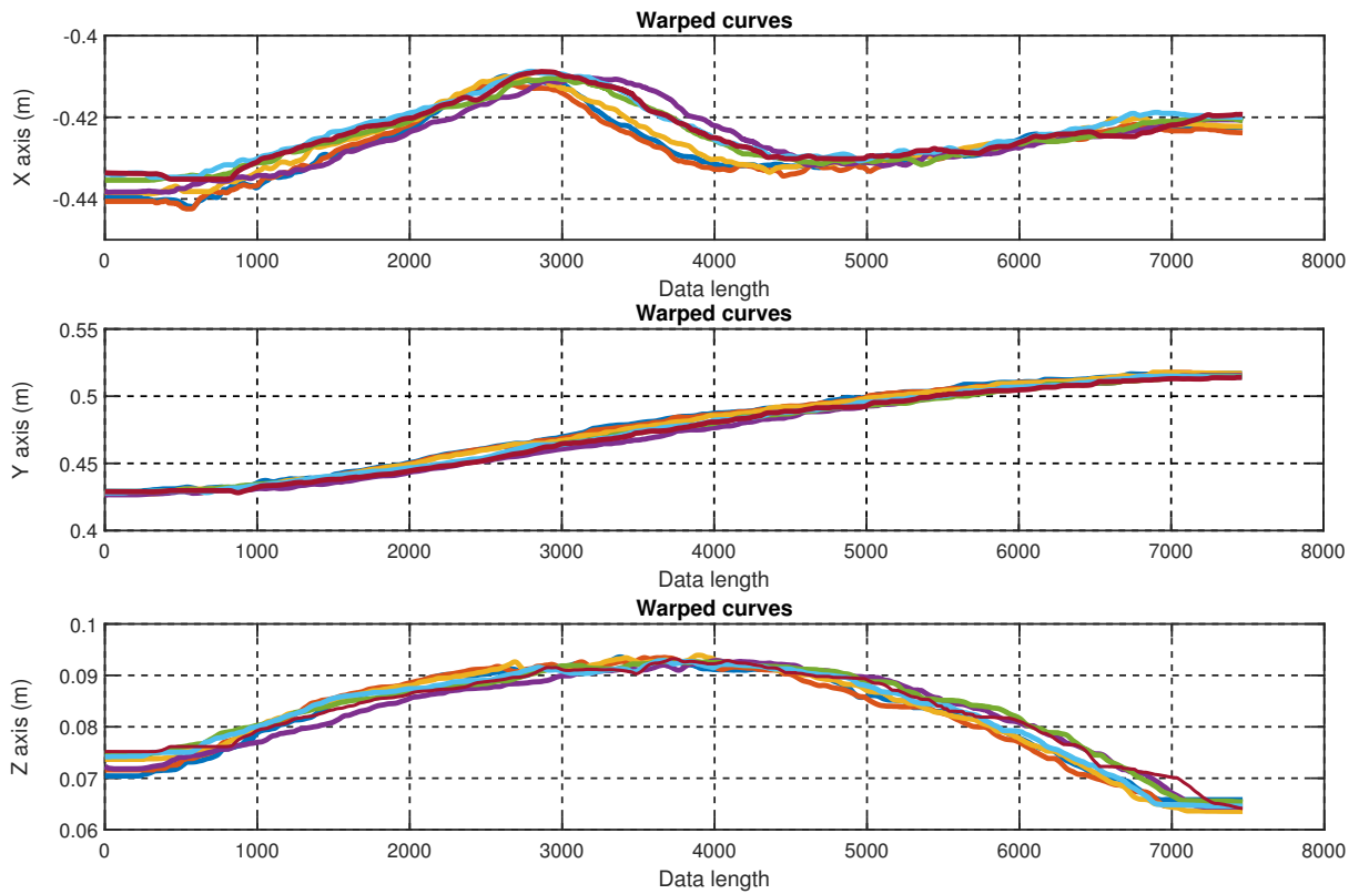
Fig. 9. Warped operation curves in 3-axis. The curves are warped with DTW to align the data.
