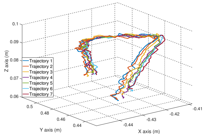
Fig. 7. Demonstrated operation curves in 3-D. The hands-on demonstrations are repeated 7 times in open surgery.
