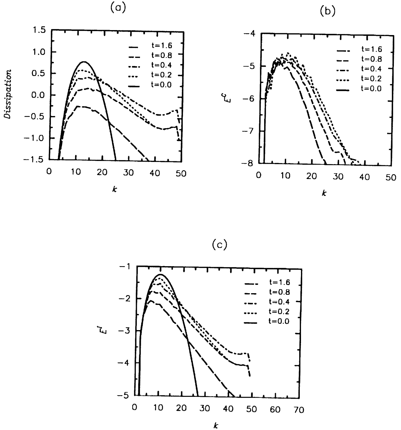
Fig. 8 Energy and dissipation spectra of 96^3 DNS at t = 0, 0.2, 0.4, 0.8, 1.6 . k_0 = 10 , \chi_0 = 0.0 , (M_t)_0 = 0.1 , (R_\lambda)_0 = 30.0 , Re = 250 . (a) Dissipation, (b) Compressible energy, (c) Solenoidal energy.
