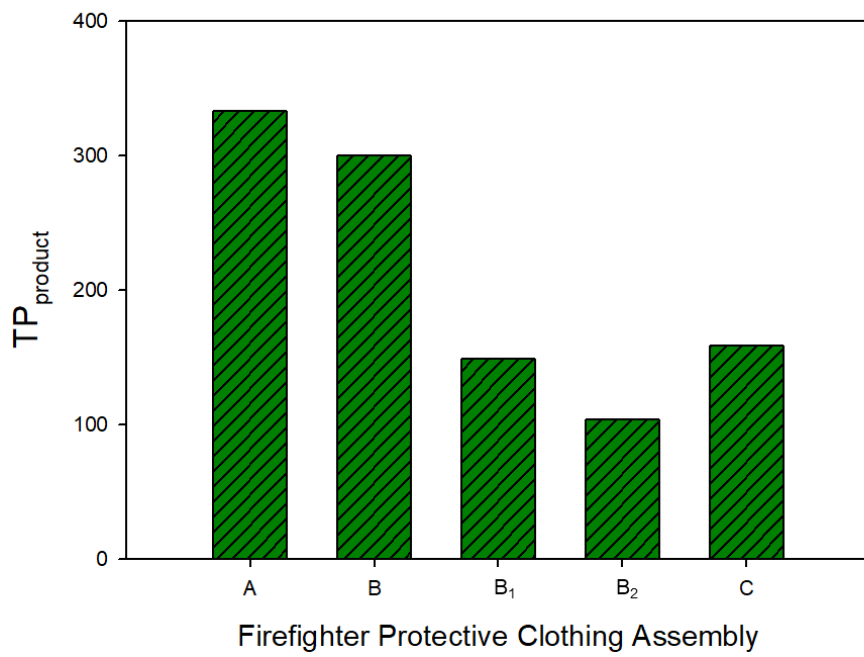
Figure 7. TP_{product} values (areas of rectangles in Figure 6) for the firefighter protective clothing assemblies.
