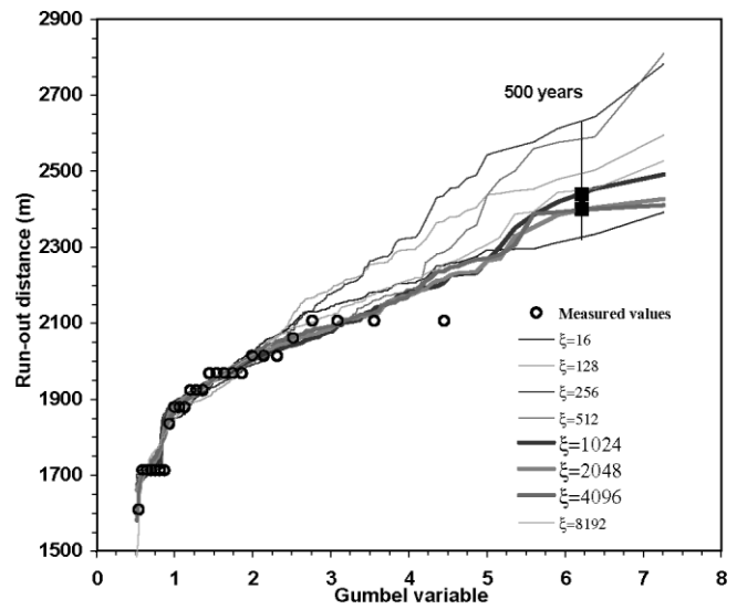
Fig. 12. Run-out distance statistical distributions with the \mu samples, different fixed values of \xi (in \text{m s}^{-2} ), and the modified profile (Voellmy-like model).
