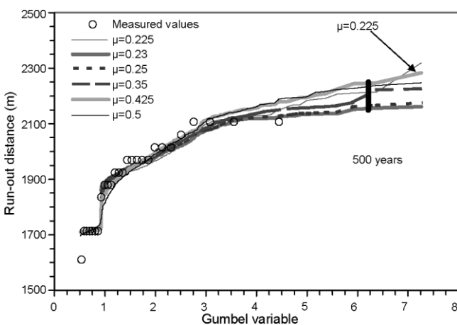
Fig. 11. Run-out distance statistical distributions with the \xi samples (in \text{m s}^{-2} ), different fixed values of \mu , and the real profile (Voellmy-like model).
