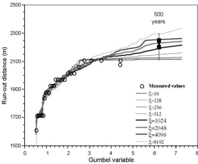
Fig. 10. Run-out distance statistical distributions with the \mu samples, different fixed values of \xi (in \text{m s}^{-2} ), and the real profile (Voellmy-like model).
