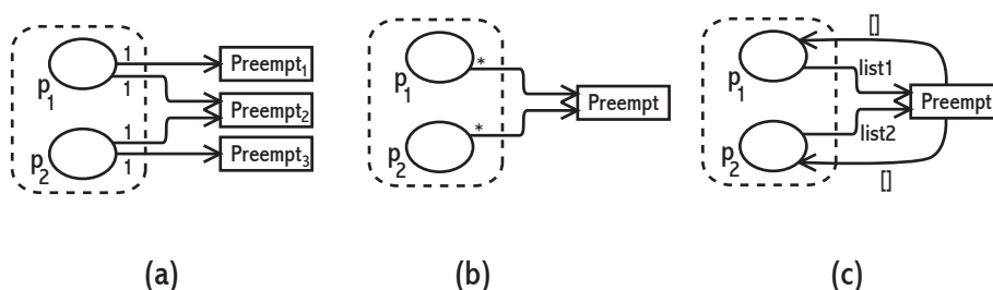
Abbildung 4: Possibilities for preempting a subnet: an individual transition for each marking (a), flush-arcs (b), and high-level nets with list-typed markings (c).
